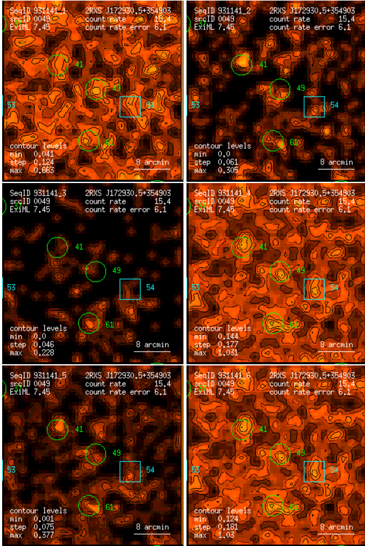
Figure 49: RASS 931141: detection 0049: band rate images, Gaussian filter: (1) PSPC channels 11 – 41, (2) 52 – 90, (3) 91 – 201, (4) 11 – 235, (5) 52 – 201, (6) 11 – 201. Broad band rates in counts/ks. Band rate contour levels in counts/ks/arcmin 2 .
