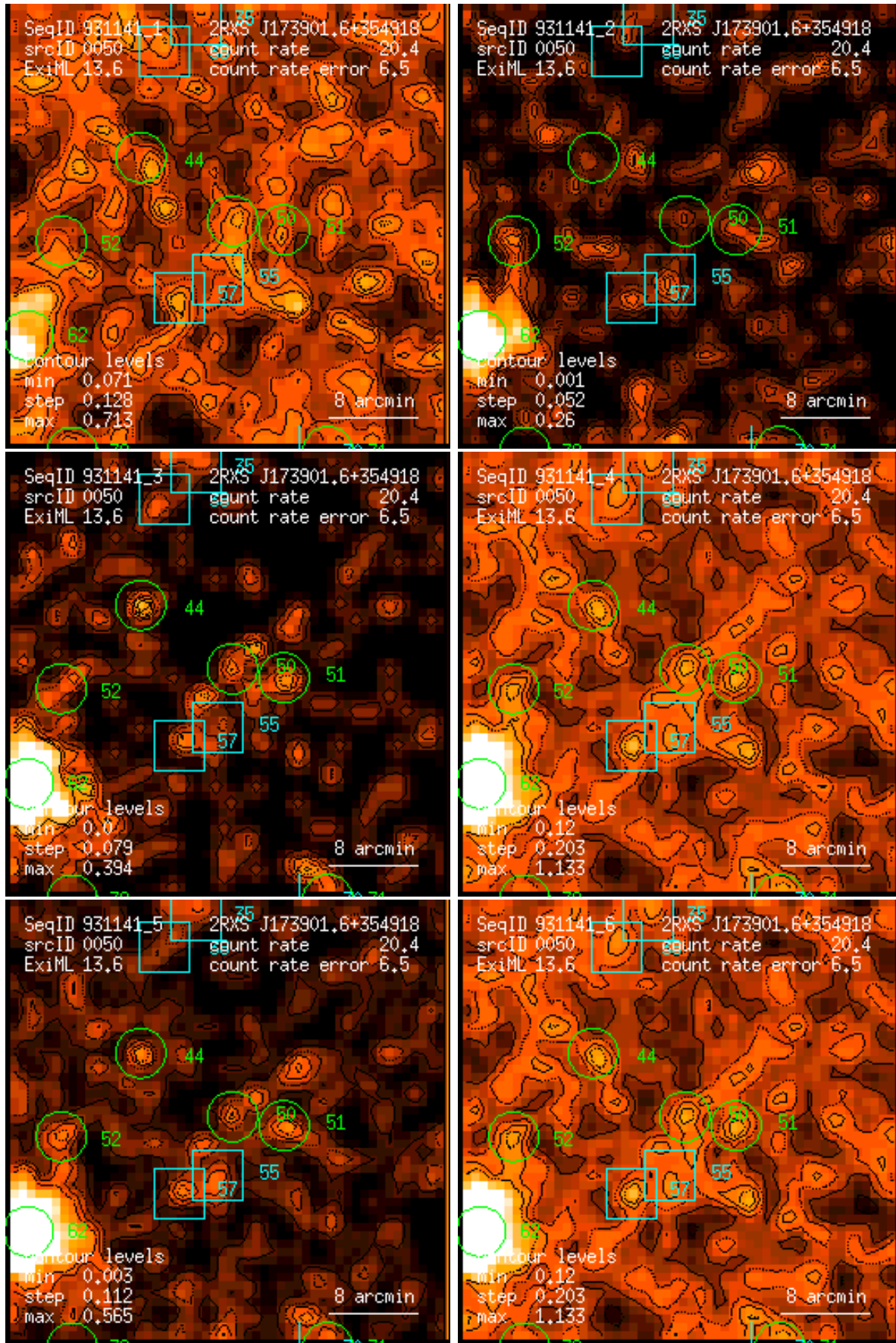
Figure 50: RASS 931141: detection 0050: band rate images, Gaussian filter: (1) PSPC channels 11 – 41, (2) 52 – 90, (3) 91 – 201, (4) 11 – 235, (5) 52 – 201, (6) 11 – 201. Broad band rates in counts/ks. Band rate contour levels in counts/ks/arcmin 2 .
