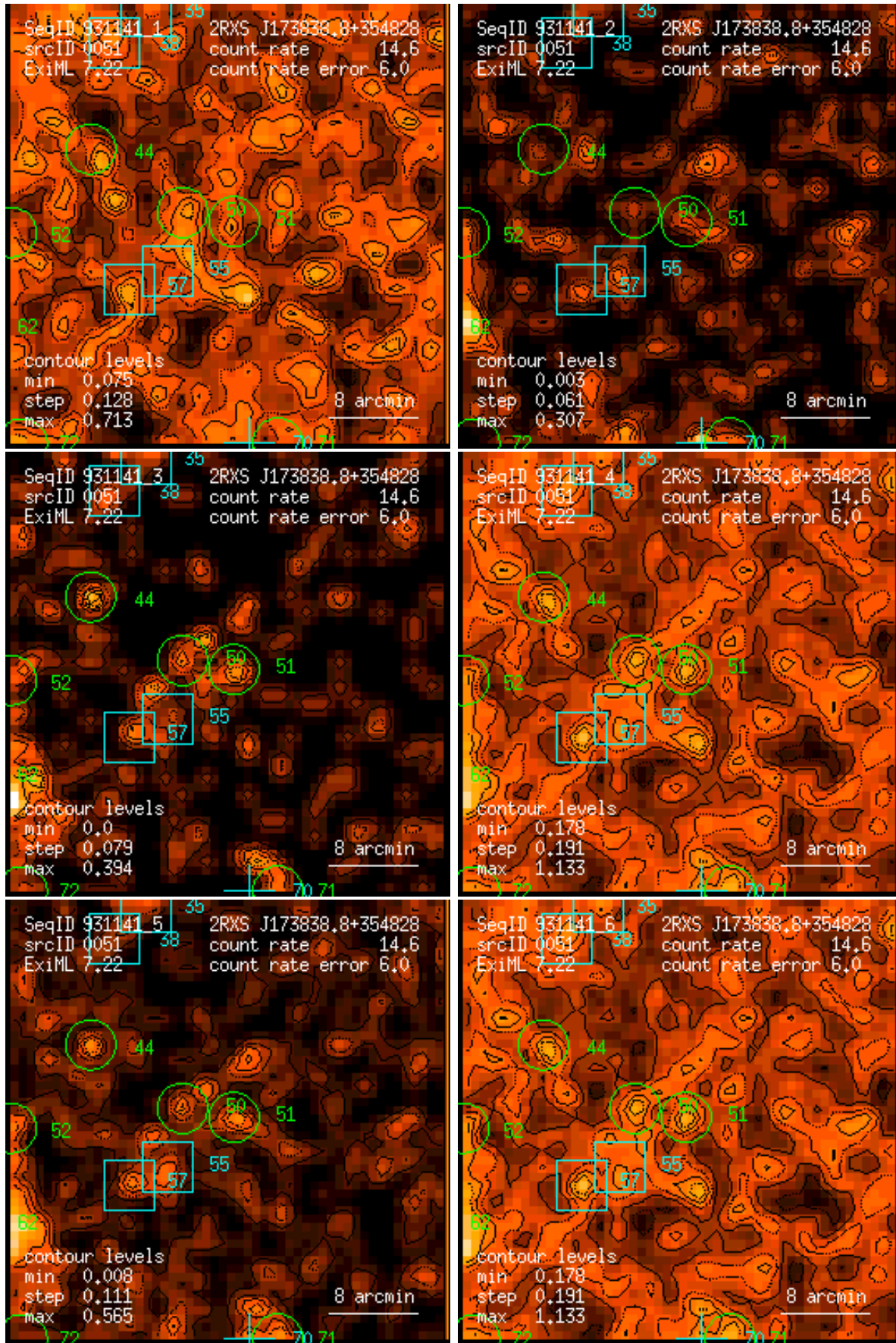
Figure 51: RASS 931141: detection 0051: band rate images, Gaussian filter: (1) PSPC channels 11 – 41, (2) 52 – 90, (3) 91 – 201, (4) 11 – 235, (5) 52 – 201, (6) 11 – 201. Broad band rates in counts/ks. Band rate contour levels in counts/ks/arcmin 2 .
