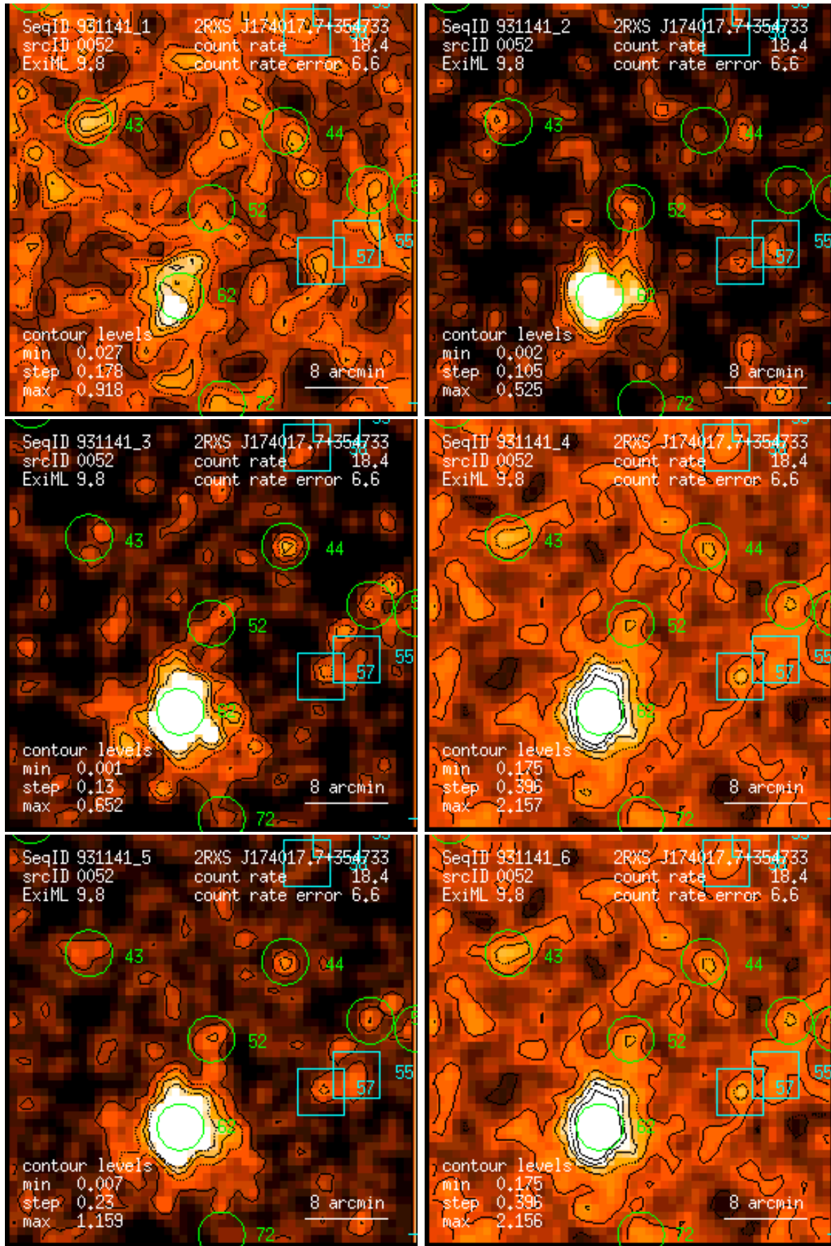
Figure 52: RASS 931141: detection 0052: band rate images, Gaussian filter: (1) PSPC channels 11 – 41, (2) 52 – 90, (3) 91 – 201, (4) 11 – 235, (5) 52 – 201, (6) 11 – 201. Broad band rates in counts/ks. Band rate contour levels in counts/ks/arcmin 2 .
