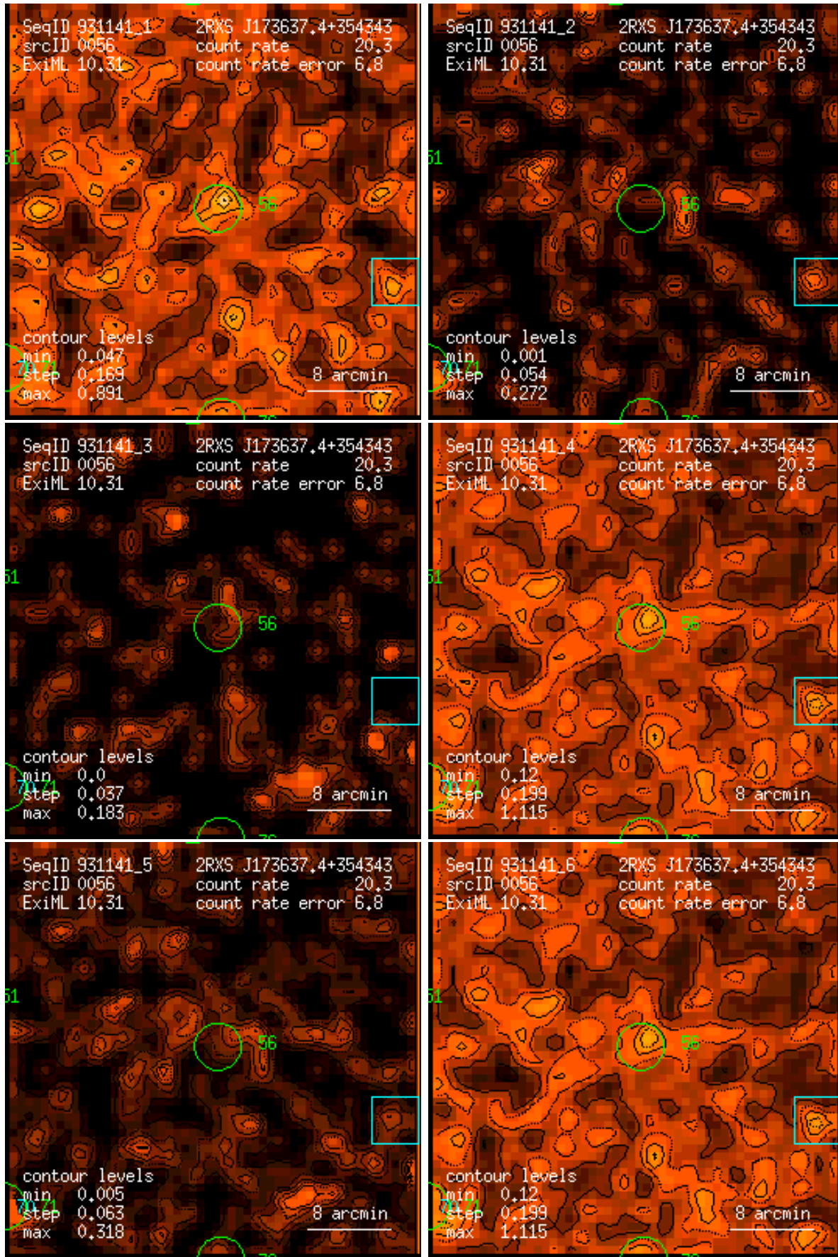
Figure 56: RASS 931141: detection 0056: band rate images, Gaussian filter: (1) PSPC channels 11 – 41, (2) 52 – 90, (3) 91 – 201, (4) 11 – 235, (5) 52 – 201, (6) 11 – 201. Broad band rates in counts/ks. Band rate contour levels in counts/ks/arcmin 2 .
