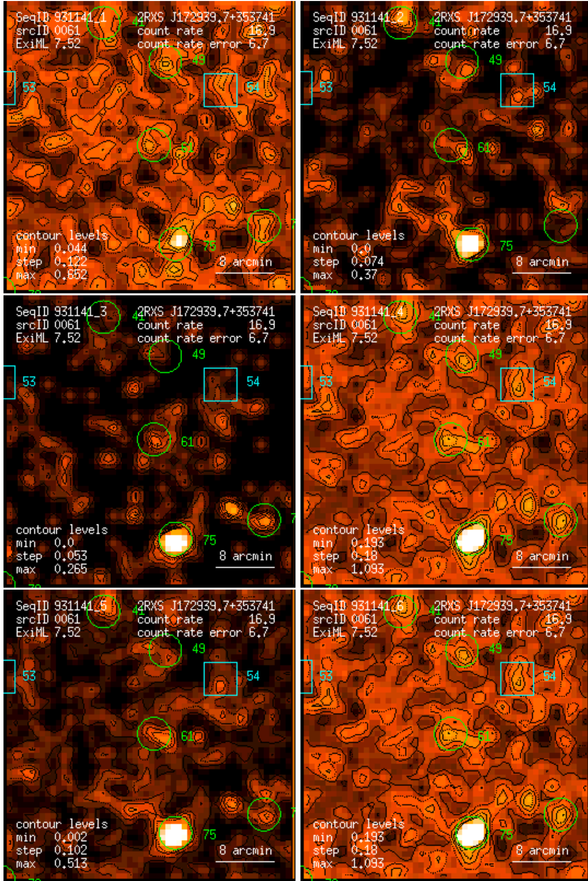
Figure 61: RASS 931141: detection 0061: band rate images, Gaussian filter: (1) PSPC channels 11 – 41, (2) 52 – 90, (3) 91 – 201, (4) 11 – 235, (5) 52 – 201, (6) 11 – 201. Broad band rates in counts/ks. Band rate contour levels in counts/ks/arcmin 2 .
