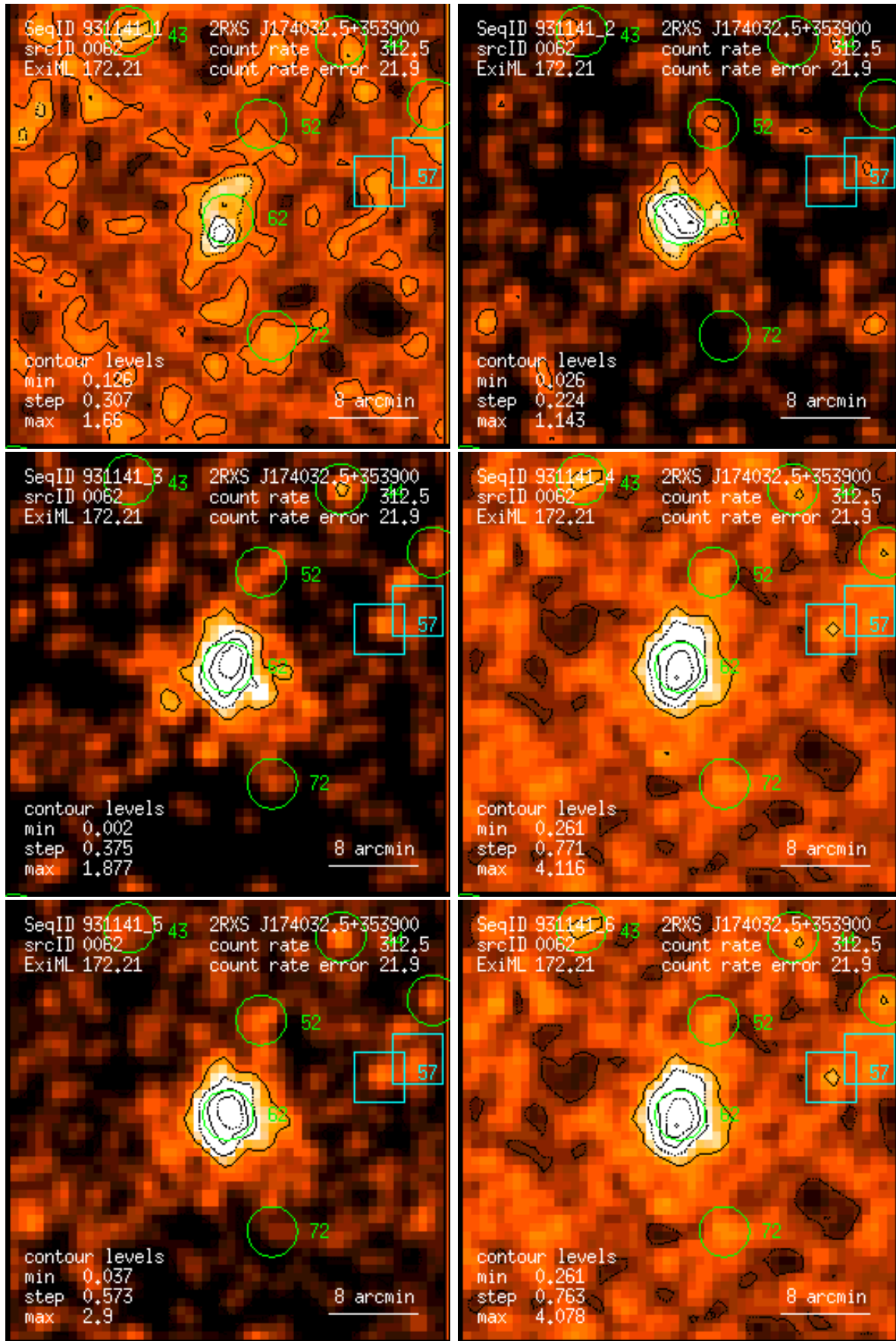
Figure 62: RASS 931141: detection 0062: band rate images, Gaussian filter: (1) PSPC channels 11 – 41, (2) 52 – 90, (3) 91 – 201, (4) 11 – 235, (5) 52 – 201, (6) 11 – 201. Broad band rates in counts/ks. Band rate contour levels in counts/ks/arcmin 2 .
