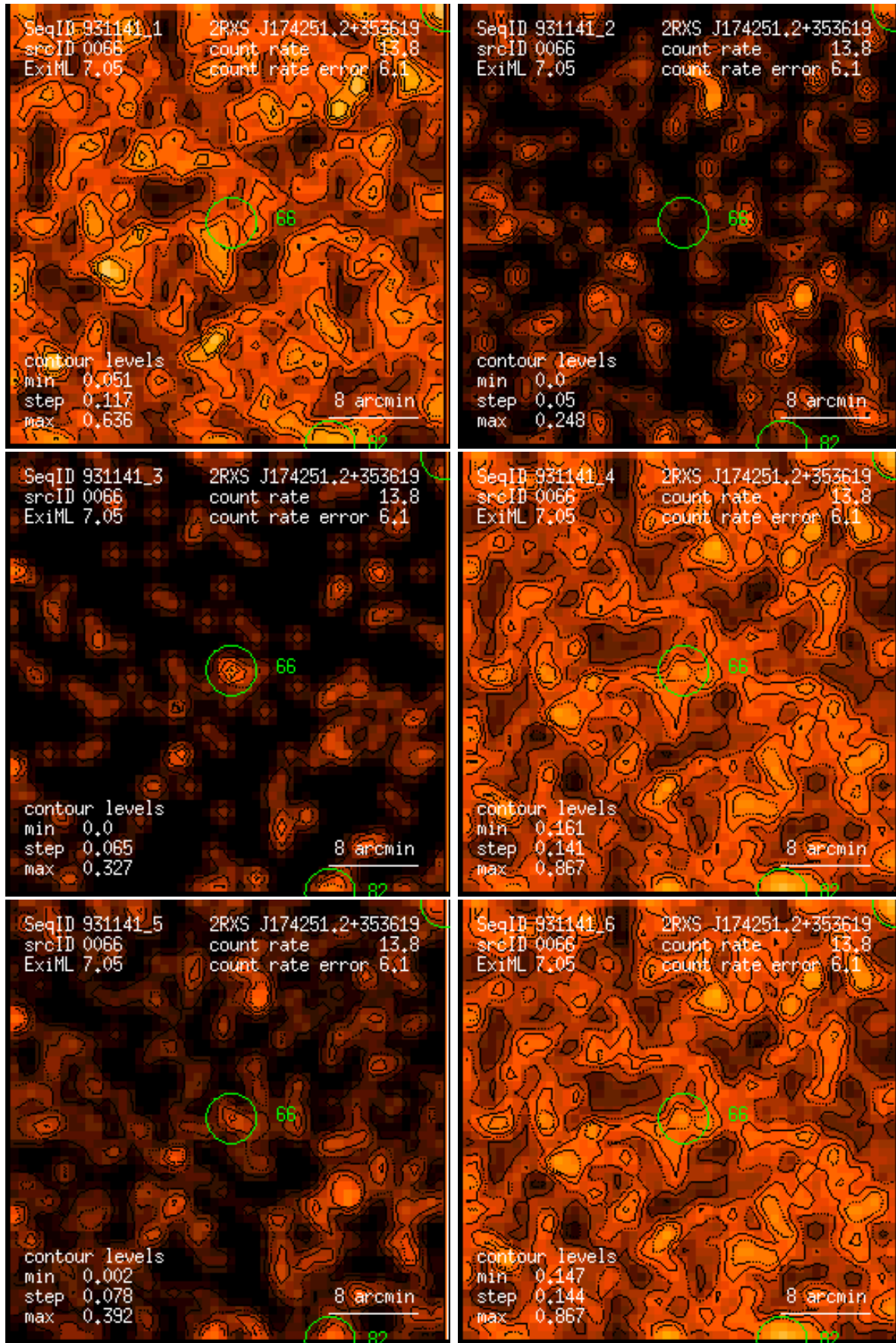
Figure 66: RASS 931141: detection 0066: band rate images, Gaussian filter: (1) PSPC channels 11 – 41, (2) 52 – 90, (3) 91 – 201, (4) 11 – 235, (5) 52 – 201, (6) 11 – 201. Broad band rates in counts/ks. Band rate contour levels in counts/ks/arcmin 2 .
