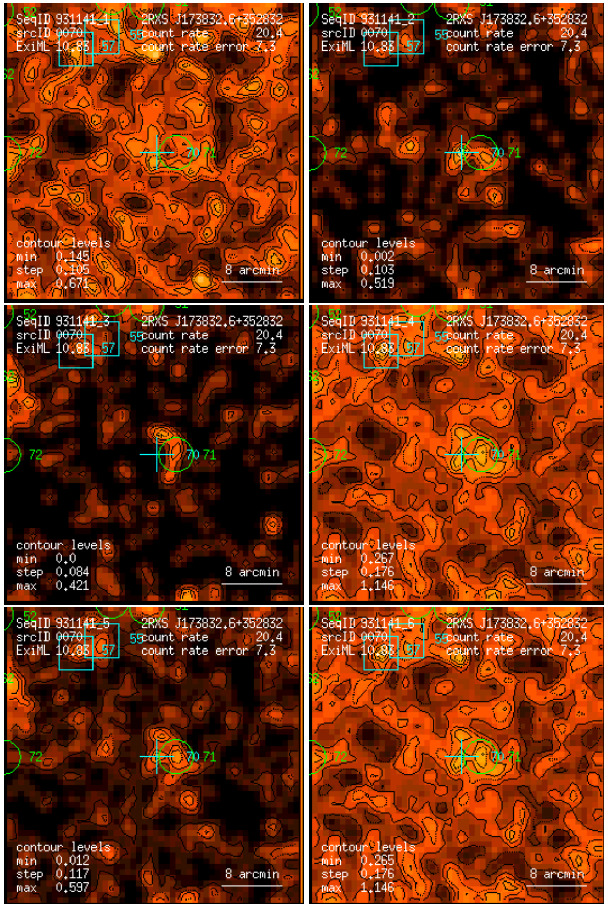
Figure 70: RASS 931141: detection 0070: band rate images, Gaussian filter: (1) PSPC channels 11 – 41, (2) 52 – 90, (3) 91 – 201, (4) 11 – 235, (5) 52 – 201, (6) 11 – 201. Broad band rates in counts/ks. Band rate contour levels in counts/ks/arcmin 2 .
