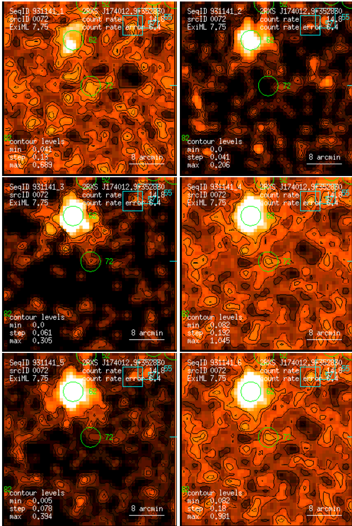
Figure 72: RASS 931141: detection 0072: band rate images, Gaussian filter: (1) PSPC channels 11 – 41, (2) 52 – 90, (3) 91 – 201, (4) 11 – 235, (5) 52 – 201, (6) 11 – 201. Broad band rates in counts/ks. Band rate contour levels in counts/ks/arcmin 2 .
