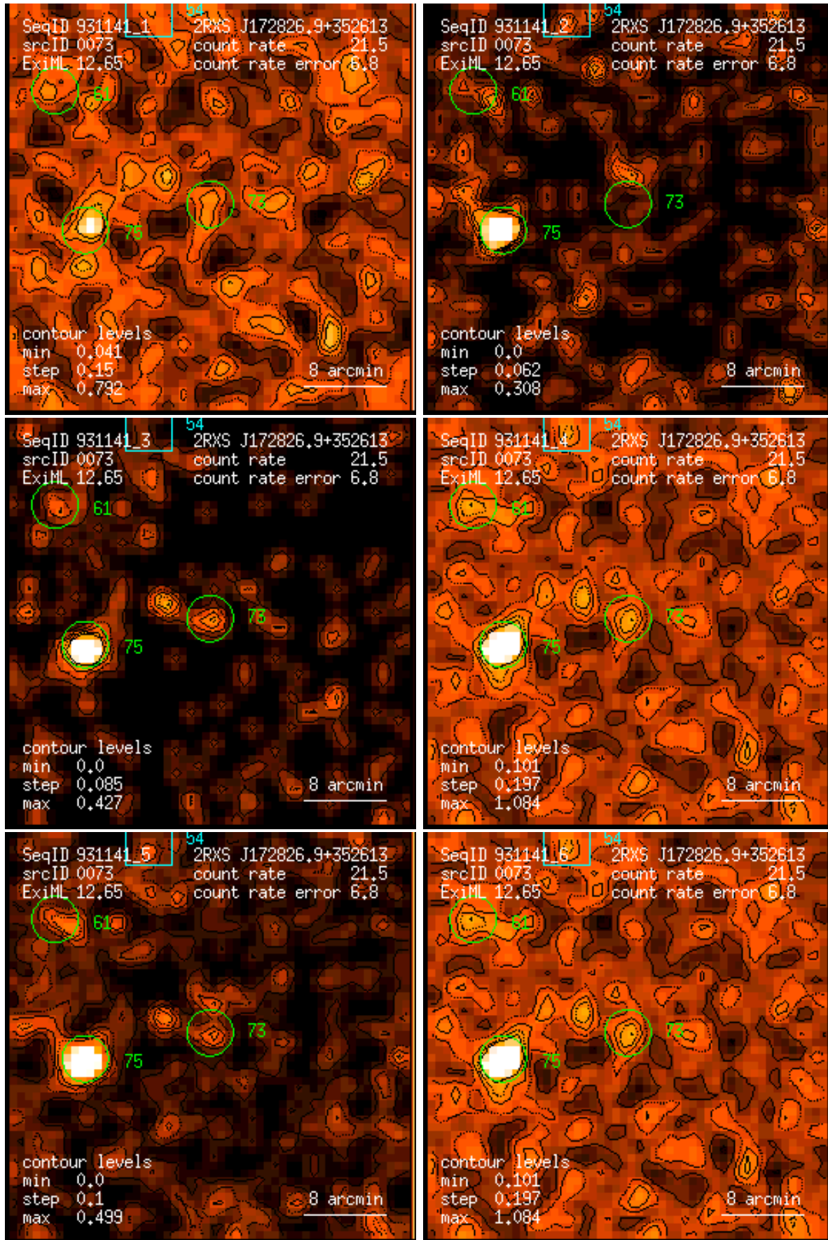
Figure 73: RASS 931141: detection 0073: band rate images, Gaussian filter: (1) PSPC channels 11 – 41, (2) 52 – 90, (3) 91 – 201, (4) 11 – 235, (5) 52 – 201, (6) 11 – 201. Broad band rates in counts/ks. Band rate contour levels in counts/ks/arcmin 2 .
