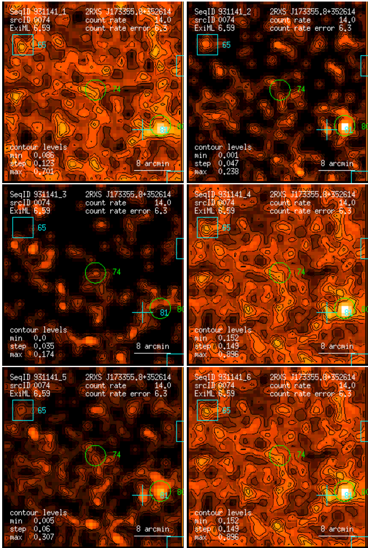
Figure 74: RASS 931141: detection 0074: band rate images, Gaussian filter: (1) PSPC channels 11 – 41, (2) 52 – 90, (3) 91 – 201, (4) 11 – 235, (5) 52 – 201, (6) 11 – 201. Broad band rates in counts/ks. Band rate contour levels in counts/ks/arcmin 2 .
