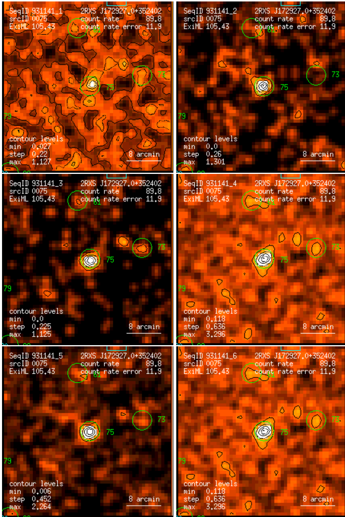
Figure 75: RASS 931141: detection 0075: band rate images, Gaussian filter: (1) PSPC channels 11 – 41, (2) 52 – 90, (3) 91 – 201, (4) 11 – 235, (5) 52 – 201, (6) 11 – 201. Broad band rates in counts/ks. Band rate contour levels in counts/ks/arcmin 2 .
