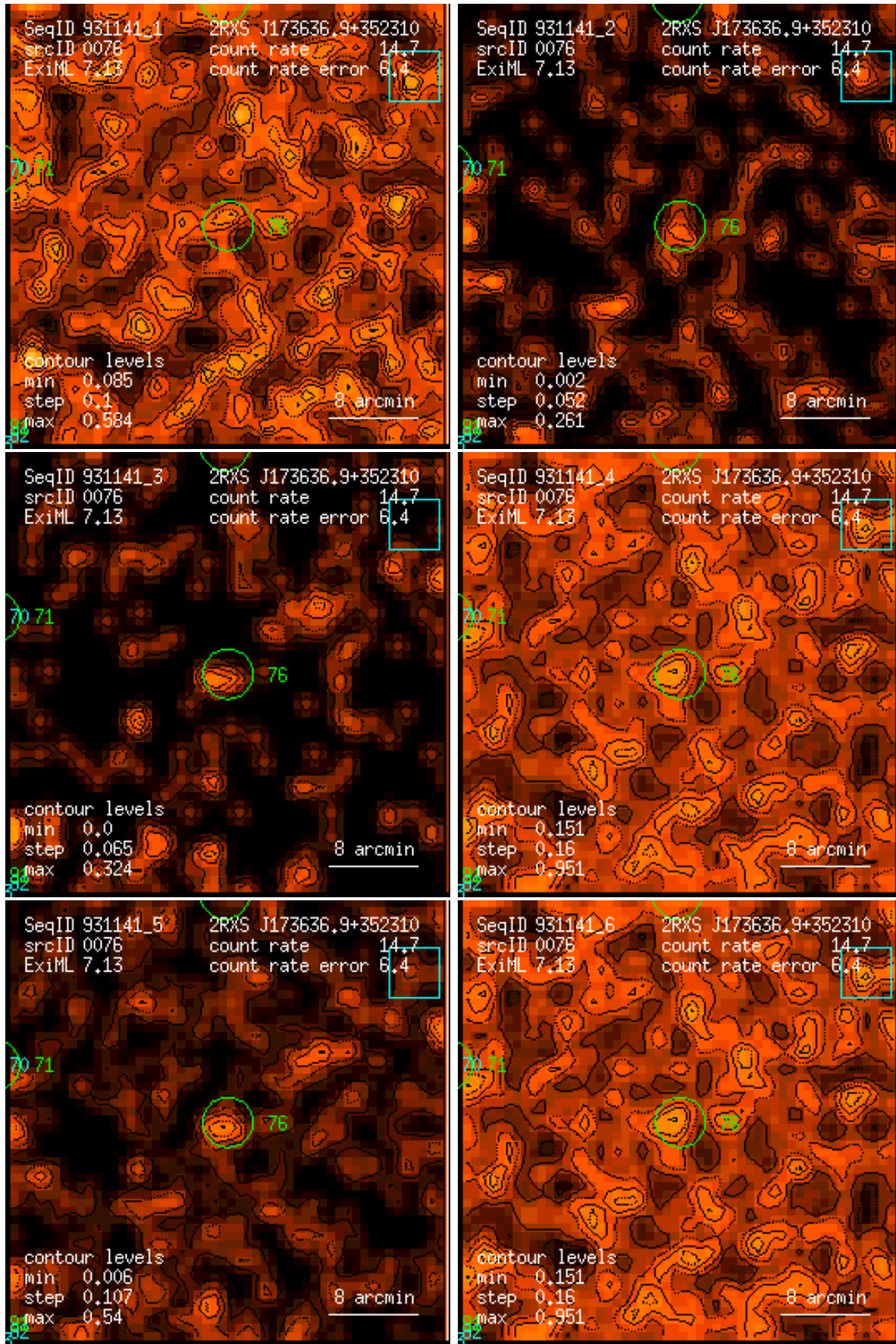
Figure 76: RASS 931141: detection 0076: band rate images, Gaussian filter: (1) PSPC channels 11 – 41, (2) 52 – 90, (3) 91 – 201, (4) 11 – 235, (5) 52 – 201, (6) 11 – 201. Broad band rates in counts/ks. Band rate contour levels in counts/ks/arcmin 2 .
