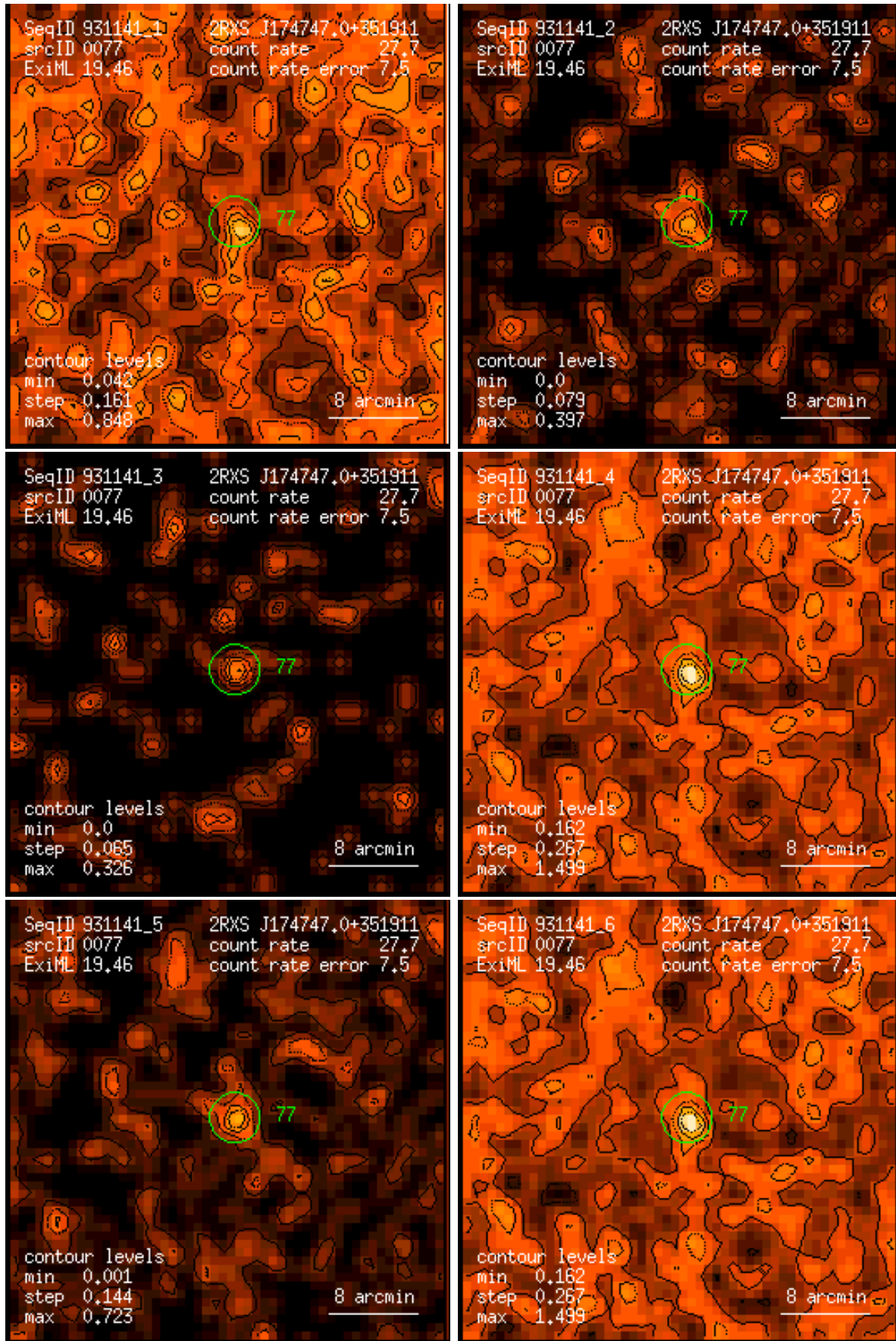
Figure 77: RASS 931141: detection 0077: band rate images, Gaussian filter: (1) PSPC channels 11 – 41, (2) 52 – 90, (3) 91 – 201, (4) 11 – 235, (5) 52 – 201, (6) 11 – 201. Broad band rates in counts/ks. Band rate contour levels in counts/ks/arcmin 2 .
