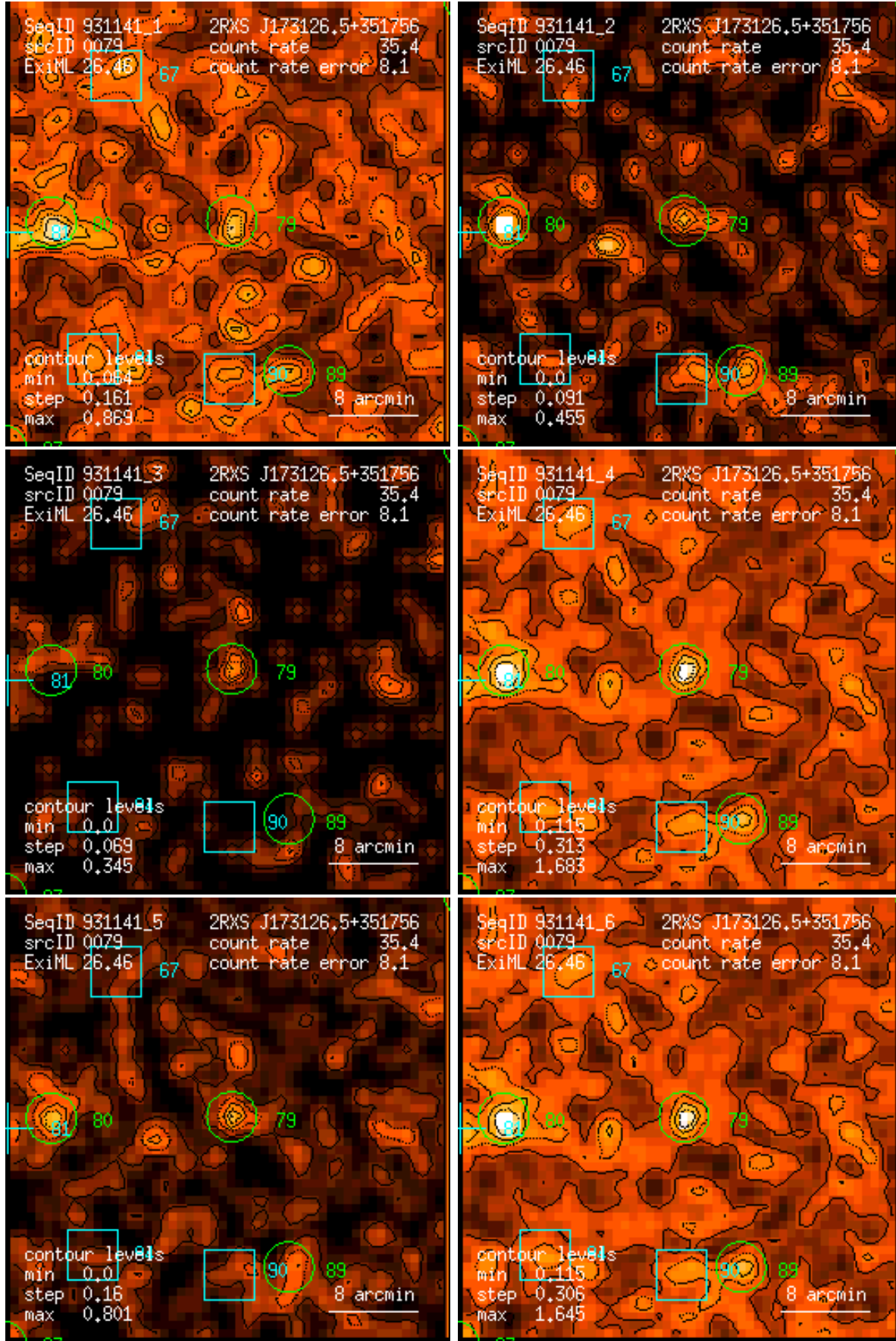
Figure 79: RASS 931141: detection 0079: band rate images, Gaussian filter: (1) PSPC channels 11 – 41, (2) 52 – 90, (3) 91 – 201, (4) 11 – 235, (5) 52 – 201, (6) 11 – 201. Broad band rates in counts/ks. Band rate contour levels in counts/ks/arcmin 2 .
