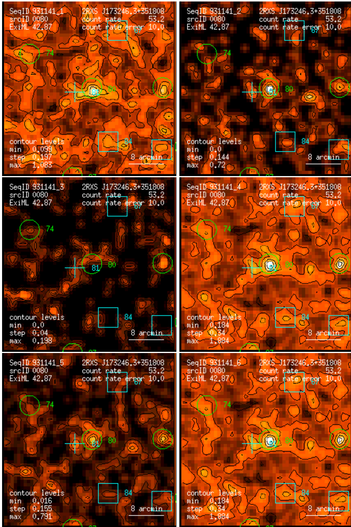
Figure 80: RASS 931141: detection 0080: band rate images, Gaussian filter: (1) PSPC channels 11 – 41, (2) 52 – 90, (3) 91 – 201, (4) 11 – 235, (5) 52 – 201, (6) 11 – 201. Broad band rates in counts/ks. Band rate contour levels in counts/ks/arcmin 2 .
