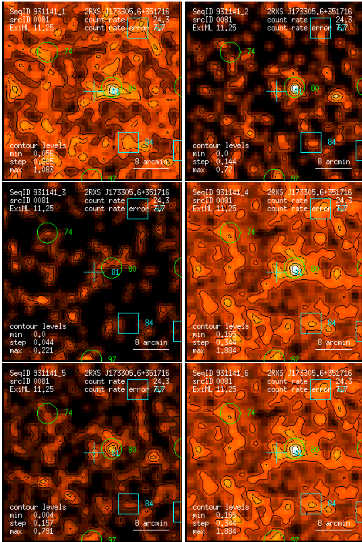
Figure 81: RASS 931141: detection 0081: band rate images, Gaussian filter: (1) PSPC channels 11 – 41, (2) 52 – 90, (3) 91 – 201, (4) 11 – 235, (5) 52 – 201, (6) 11 – 201. Broad band rates in counts/ks. Band rate contour levels in counts/ks/arcmin 2 .
