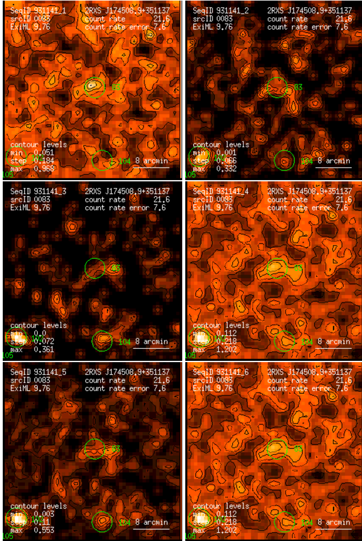
Figure 83: RASS 931141: detection 0083: band rate images, Gaussian filter: (1) PSPC channels 11 – 41, (2) 52 – 90, (3) 91 – 201, (4) 11 – 235, (5) 52 – 201, (6) 11 – 201. Broad band rates in counts/ks. Band rate contour levels in counts/ks/arcmin 2 .
