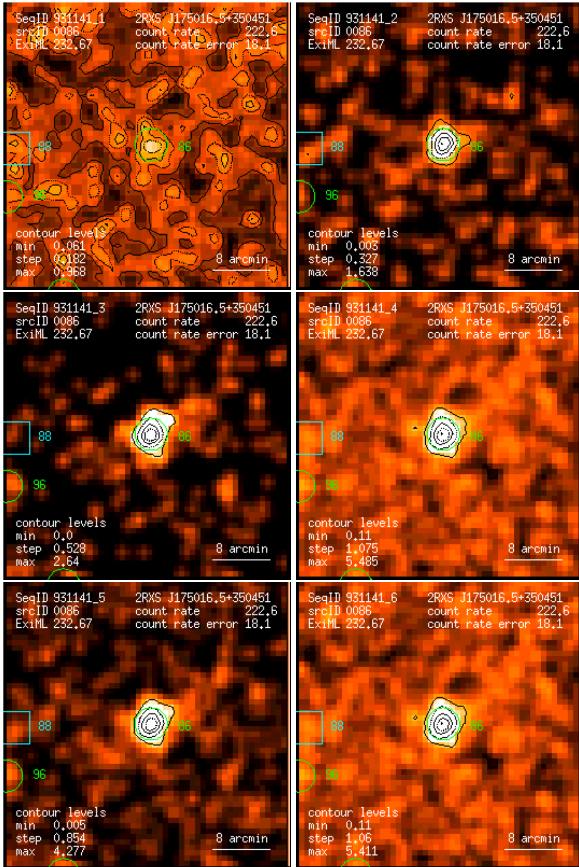
Figure 86: RASS 931141: detection 0086: band rate images, Gaussian filter: (1) PSPC channels 11 – 41, (2) 52 – 90, (3) 91 – 201, (4) 11 – 235, (5) 52 – 201, (6) 11 – 201. Broad band rates in counts/ks. Band rate contour levels in counts/ks/arcmin 2 .
