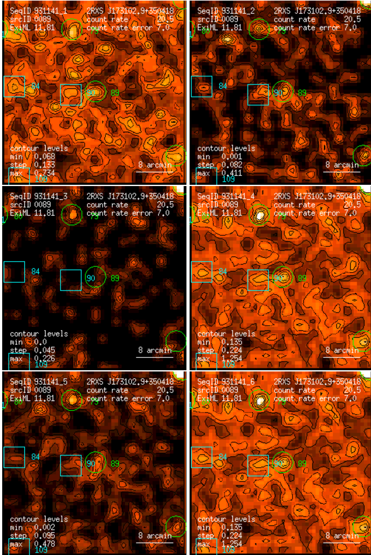
Figure 89: RASS 931141: detection 0089: band rate images, Gaussian filter: (1) PSPC channels 11 – 41, (2) 52 – 90, (3) 91 – 201, (4) 11 – 235, (5) 52 – 201, (6) 11 – 201. Broad band rates in counts/ks. Band rate contour levels in counts/ks/arcmin 2 .
