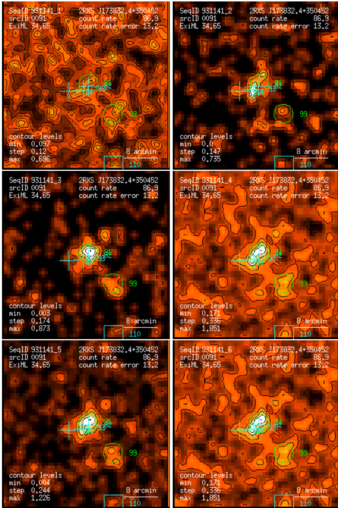
Figure 91: RASS 931141: detection 0091: band rate images, Gaussian filter: (1) PSPC channels 11 – 41, (2) 52 – 90, (3) 91 – 201, (4) 11 – 235, (5) 52 – 201, (6) 11 – 201. Broad band rates in counts/ks. Band rate contour levels in counts/ks/arcmin 2 .
