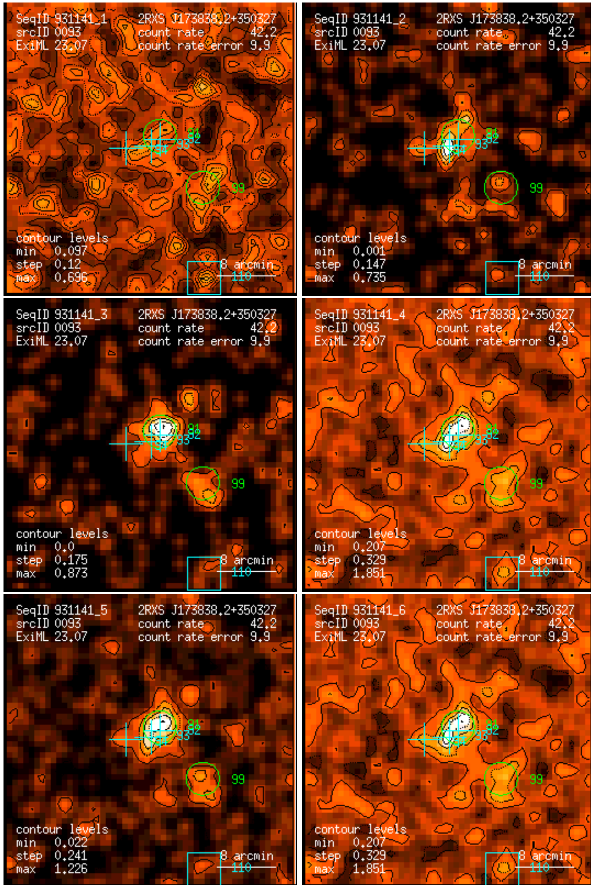
Figure 93: RASS 931141: detection 0093: band rate images, Gaussian filter: (1) PSPC channels 11 – 41, (2) 52 – 90, (3) 91 – 201, (4) 11 – 235, (5) 52 – 201, (6) 11 – 201. Broad band rates in counts/ks. Band rate contour levels in counts/ks/arcmin 2 .
