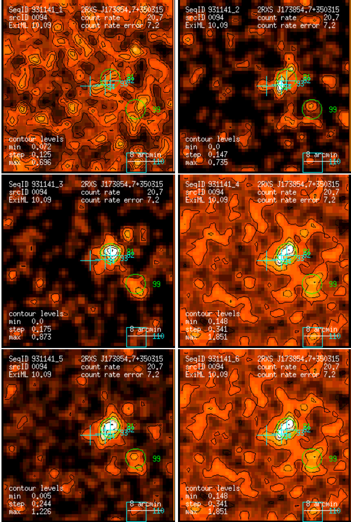
Figure 94: RASS 931141: detection 0094: band rate images, Gaussian filter: (1) PSPC channels 11 – 41, (2) 52 – 90, (3) 91 – 201, (4) 11 – 235, (5) 52 – 201, (6) 11 – 201. Broad band rates in counts/ks. Band rate contour levels in counts/ks/arcmin 2 .
