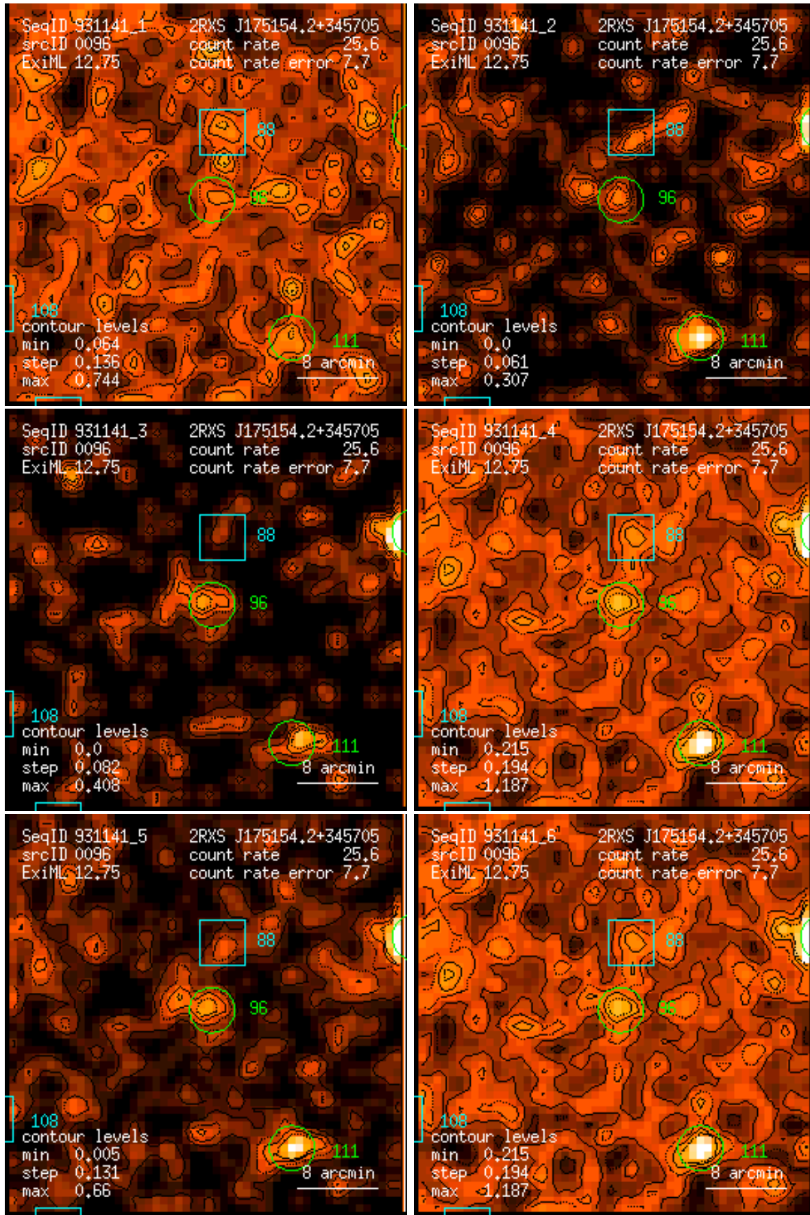
Figure 96: RASS 931141: detection 0096: band rate images, Gaussian filter: (1) PSPC channels 11 – 41, (2) 52 – 90, (3) 91 – 201, (4) 11 – 235, (5) 52 – 201, (6) 11 – 201. Broad band rates in counts/ks. Band rate contour levels in counts/ks/arcmin 2 .
