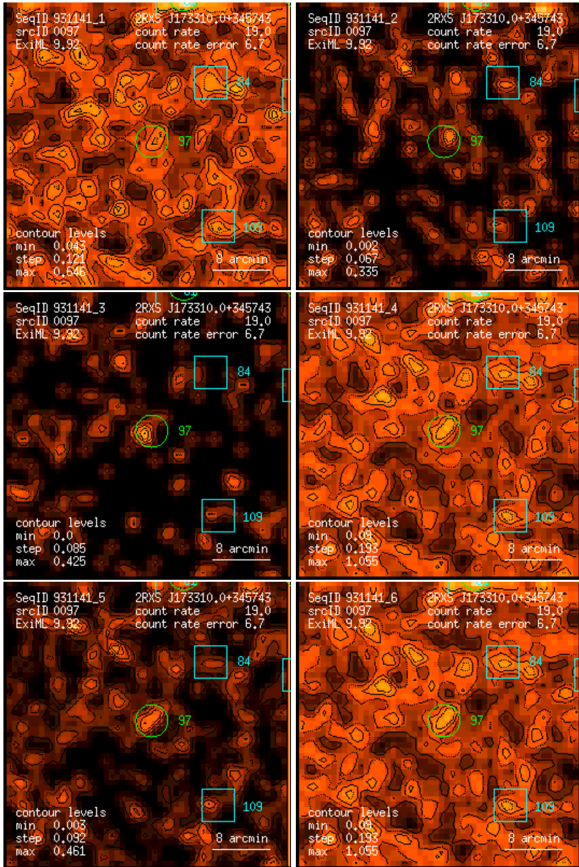
Figure 97: RASS 931141: detection 0097: band rate images, Gaussian filter: (1) PSPC channels 11 – 41, (2) 52 – 90, (3) 91 – 201, (4) 11 – 235, (5) 52 – 201, (6) 11 – 201. Broad band rates in counts/ks. Band rate contour levels in counts/ks/arcmin 2 .
