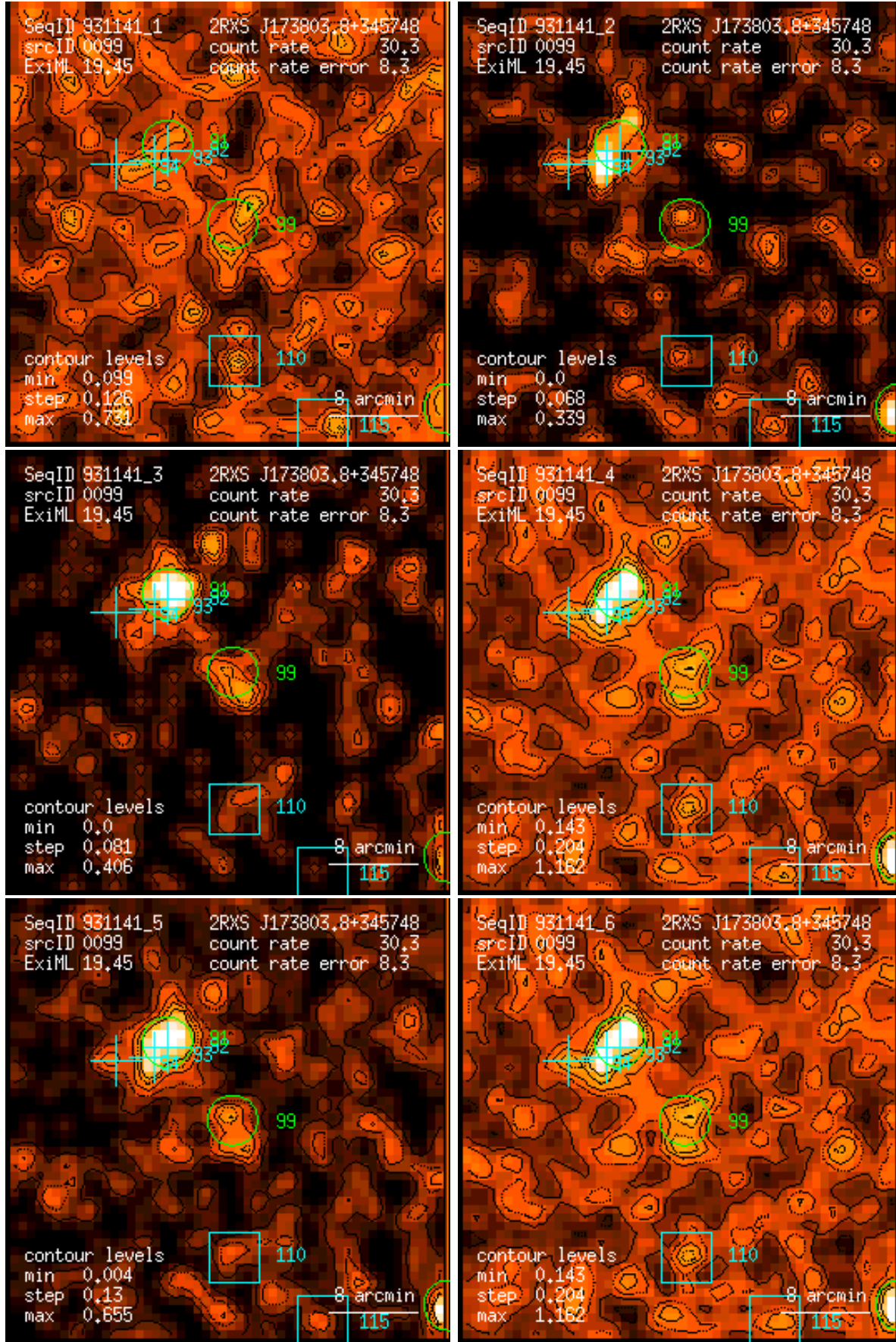
Figure 99: RASS 931141: detection 0099: band rate images, Gaussian filter: (1) PSPC channels 11 – 41, (2) 52 – 90, (3) 91 – 201, (4) 11 – 235, (5) 52 – 201, (6) 11 – 201. Broad band rates in counts/ks. Band rate contour levels in counts/ks/arcmin 2 .
