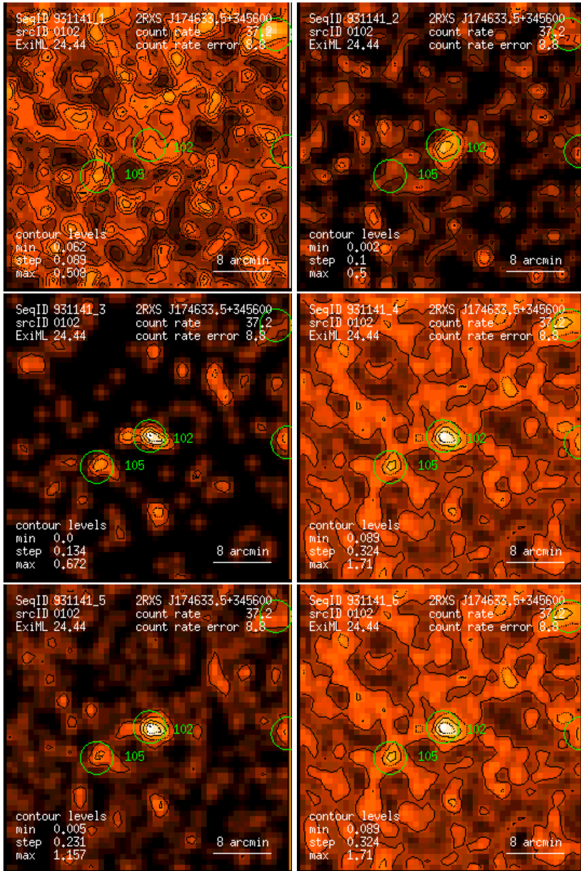
Figure 102: RASS 931141: detection 0102: band rate images, Gaussian filter: (1) PSPC channels 11 – 41, (2) 52 – 90, (3) 91 – 201, (4) 11 – 235, (5) 52 – 201, (6) 11 – 201. Broad band rates in counts/ks. Band rate contour levels in counts/ks/arcmin 2 .
