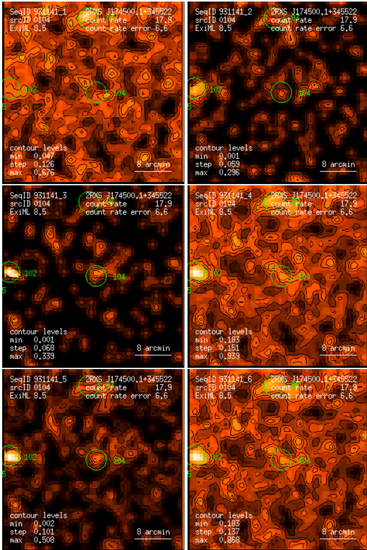
Figure 104: RASS 931141: detection 0104: band rate images, Gaussian filter: (1) PSPC channels 11 – 41, (2) 52 – 90, (3) 91 – 201, (4) 11 – 235, (5) 52 – 201, (6) 11 – 201. Broad band rates in counts/ks. Band rate contour levels in counts/ks/arcmin 2 .
