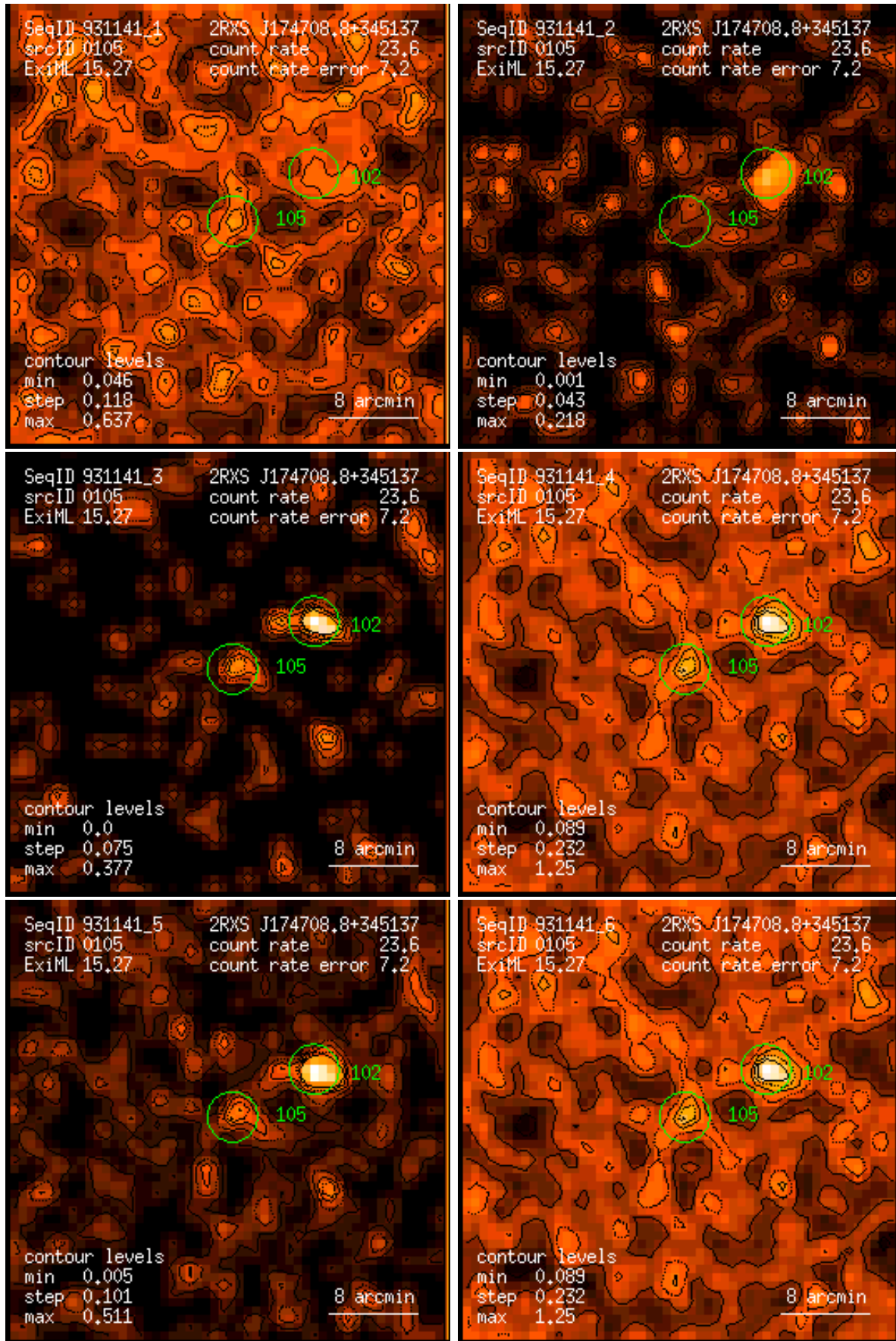
Figure 105: RASS 931141: detection 0105: band rate images, Gaussian filter: (1) PSPC channels 11 – 41, (2) 52 – 90, (3) 91 – 201, (4) 11 – 235, (5) 52 – 201, (6) 11 – 201. Broad band rates in counts/ks. Band rate contour levels in counts/ks/arcmin 2 .
