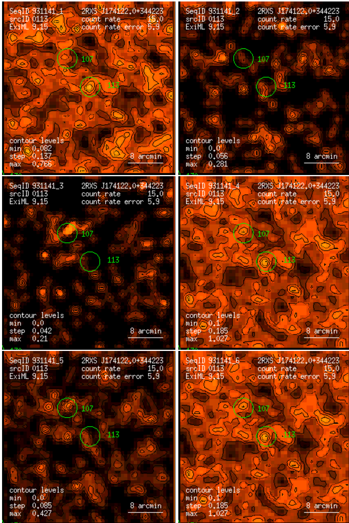
Figure 113: RASS 931141: detection 0113: band rate images, Gaussian filter: (1) PSPC channels 11 – 41, (2) 52 – 90, (3) 91 – 201, (4) 11 – 235, (5) 52 – 201, (6) 11 – 201. Broad band rates in counts/ks. Band rate contour levels in counts/ks/arcmin 2 .
