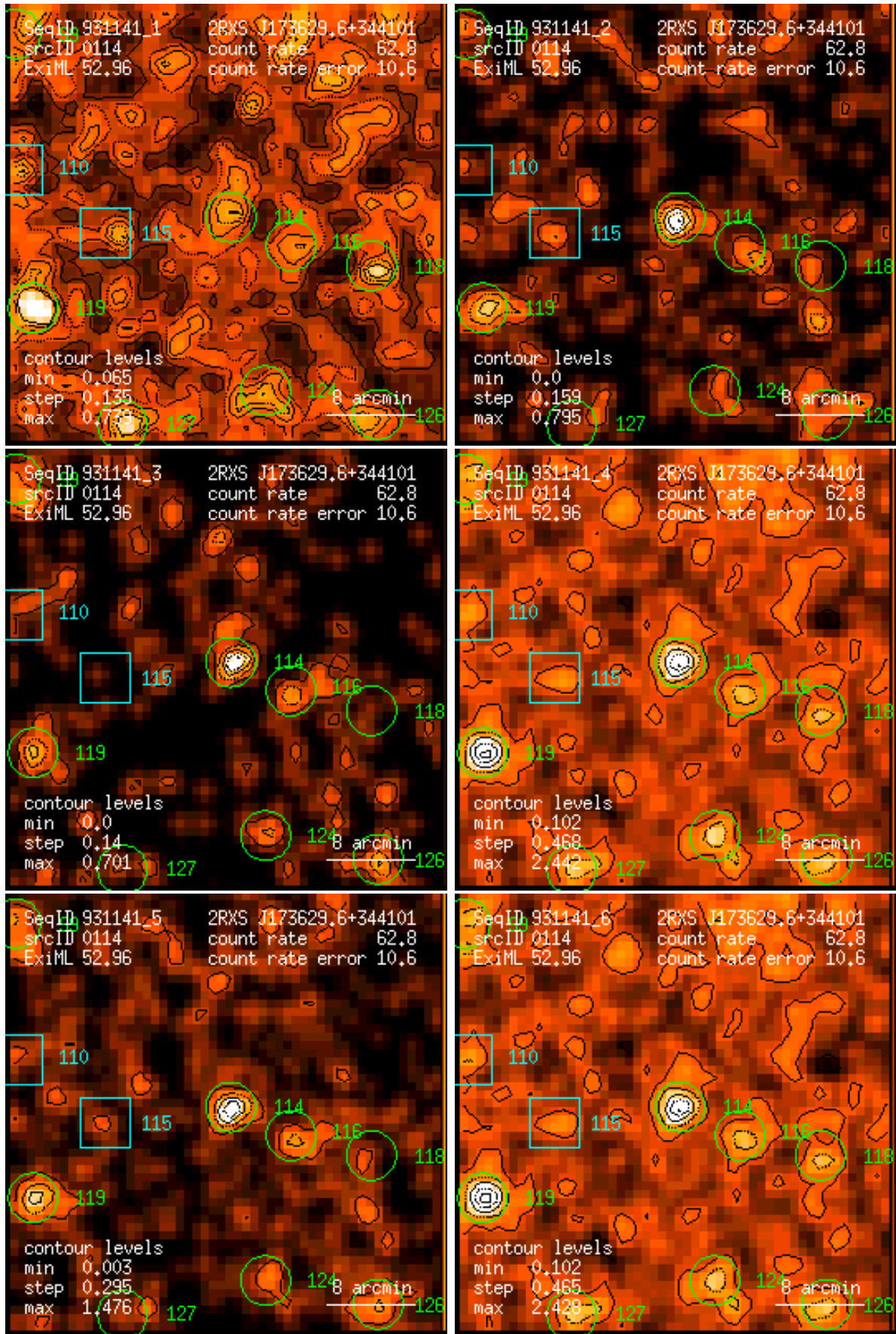
Figure 114: RASS 931141: detection 0114: band rate images, Gaussian filter: (1) PSPC channels 11 – 41, (2) 52 – 90, (3) 91 – 201, (4) 11 – 235, (5) 52 – 201, (6) 11 – 201. Broad band rates in counts/ks. Band rate contour levels in counts/ks/arcmin 2 .
