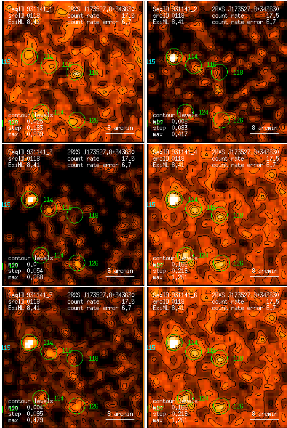
Figure 118: RASS 931141: detection 0118: band rate images, Gaussian filter: (1) PSPC channels 11 – 41, (2) 52 – 90, (3) 91 – 201, (4) 11 – 235, (5) 52 – 201, (6) 11 – 201. Broad band rates in counts/ks. Band rate contour levels in counts/ks/arcmin 2 .
