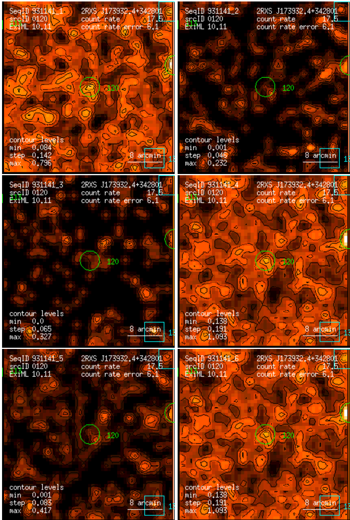
Figure 120: RASS 931141: detection 0120: band rate images, Gaussian filter: (1) PSPC channels 11 – 41, (2) 52 – 90, (3) 91 – 201, (4) 11 – 235, (5) 52 – 201, (6) 11 – 201. Broad band rates in counts/ks. Band rate contour levels in counts/ks/arcmin 2 .
