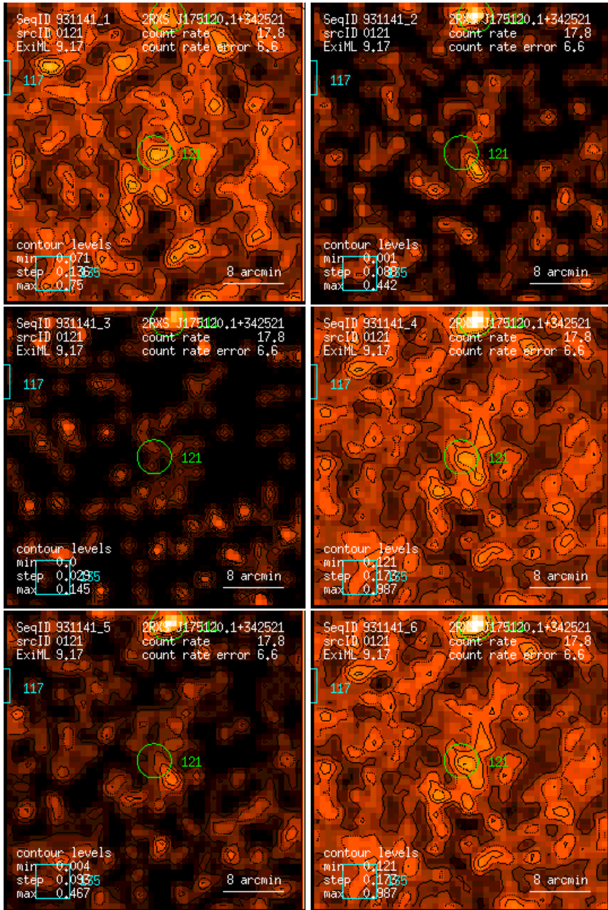
Figure 121: RASS 931141: detection 0121: band rate images, Gaussian filter: (1) PSPC channels 11 – 41, (2) 52 – 90, (3) 91 – 201, (4) 11 – 235, (5) 52 – 201, (6) 11 – 201. Broad band rates in counts/ks. Band rate contour levels in counts/ks/arcmin 2 .
