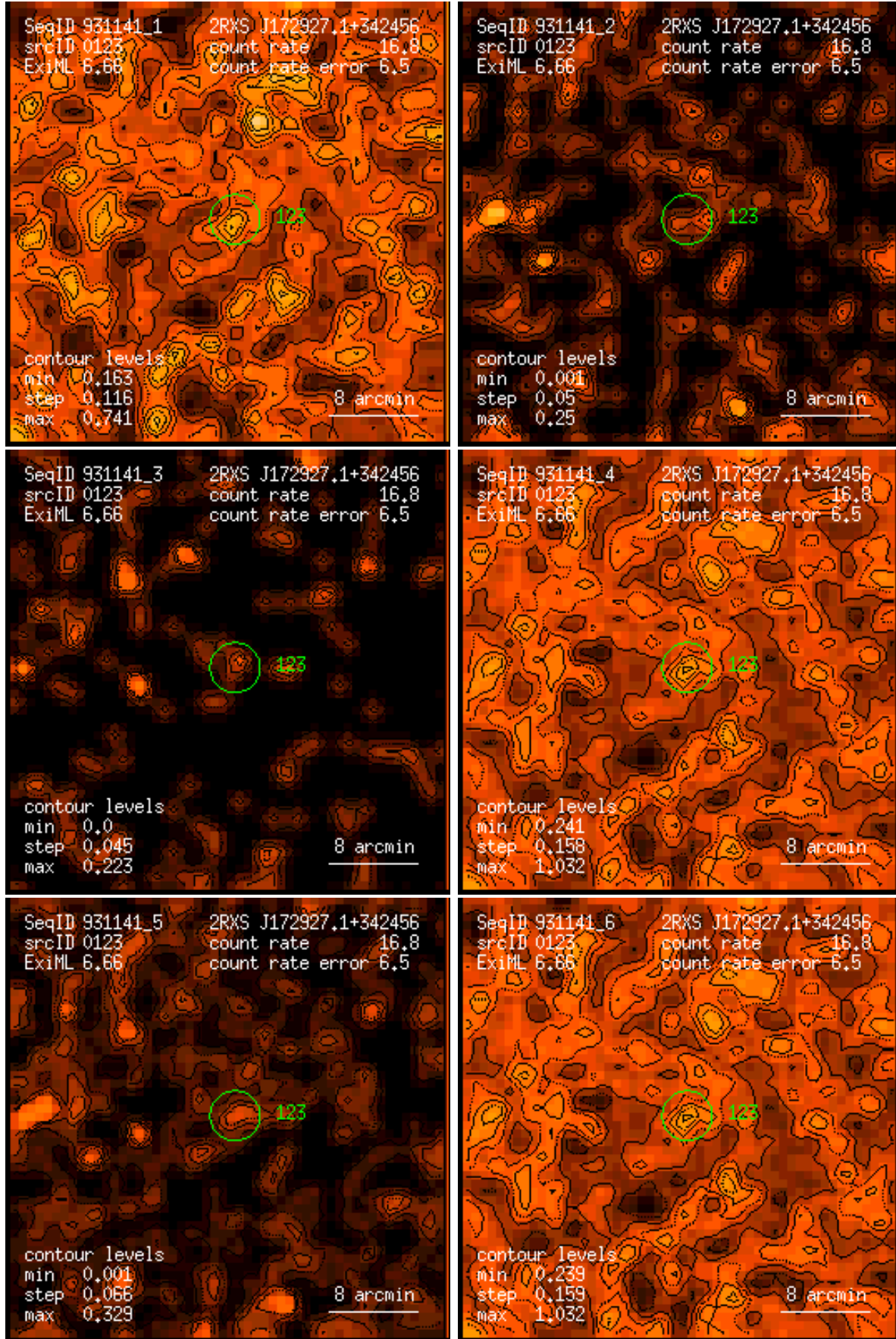
Figure 123: RASS 931141: detection 0123: band rate images, Gaussian filter: (1) PSPC channels 11 – 41, (2) 52 – 90, (3) 91 – 201, (4) 11 – 235, (5) 52 – 201, (6) 11 – 201. Broad band rates in counts/ks. Band rate contour levels in counts/ks/arcmin 2 .
