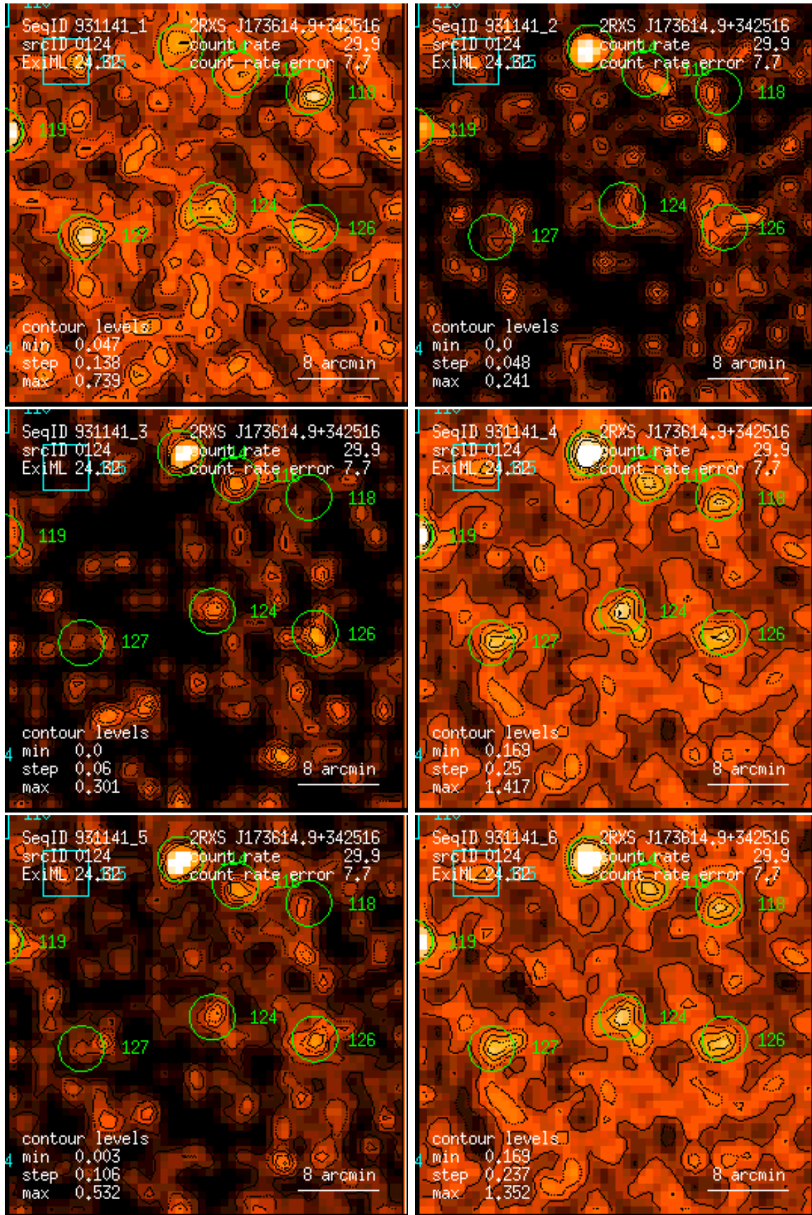
Figure 124: RASS 931141: detection 0124: band rate images, Gaussian filter: (1) PSPC channels 11 – 41, (2) 52 – 90, (3) 91 – 201, (4) 11 – 235, (5) 52 – 201, (6) 11 – 201. Broad band rates in counts/ks. Band rate contour levels in counts/ks/arcmin 2 .
