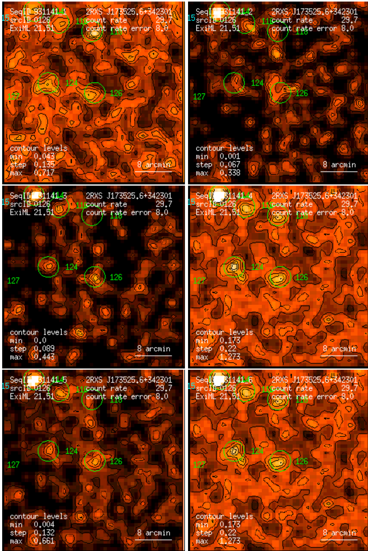
Figure 126: RASS 931141: detection 0126: band rate images, Gaussian filter: (1) PSPC channels 11 – 41, (2) 52 – 90, (3) 91 – 201, (4) 11 – 235, (5) 52 – 201, (6) 11 – 201. Broad band rates in counts/ks. Band rate contour levels in counts/ks/arcmin 2 .
