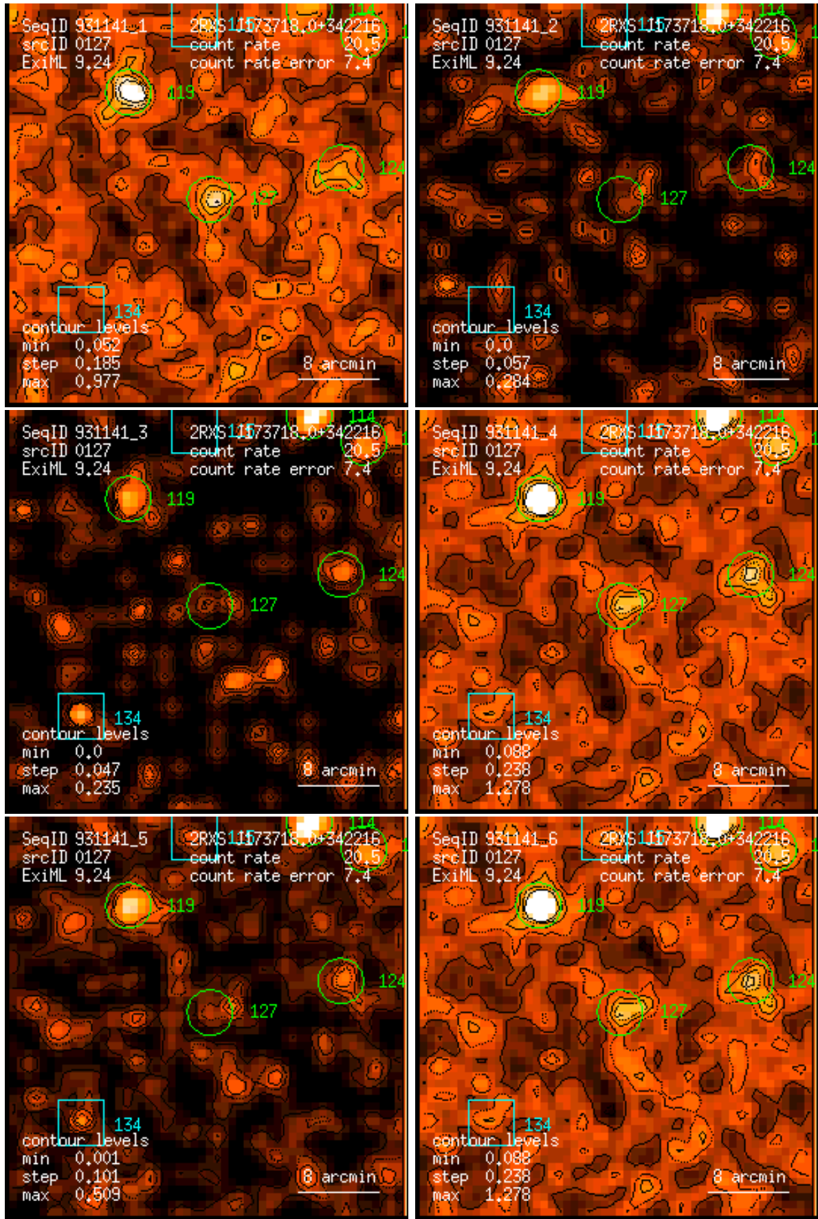
Figure 127: RASS 931141: detection 0127: band rate images, Gaussian filter: (1) PSPC channels 11 – 41, (2) 52 – 90, (3) 91 – 201, (4) 11 – 235, (5) 52 – 201, (6) 11 – 201. Broad band rates in counts/ks. Band rate contour levels in counts/ks/arcmin 2 .
