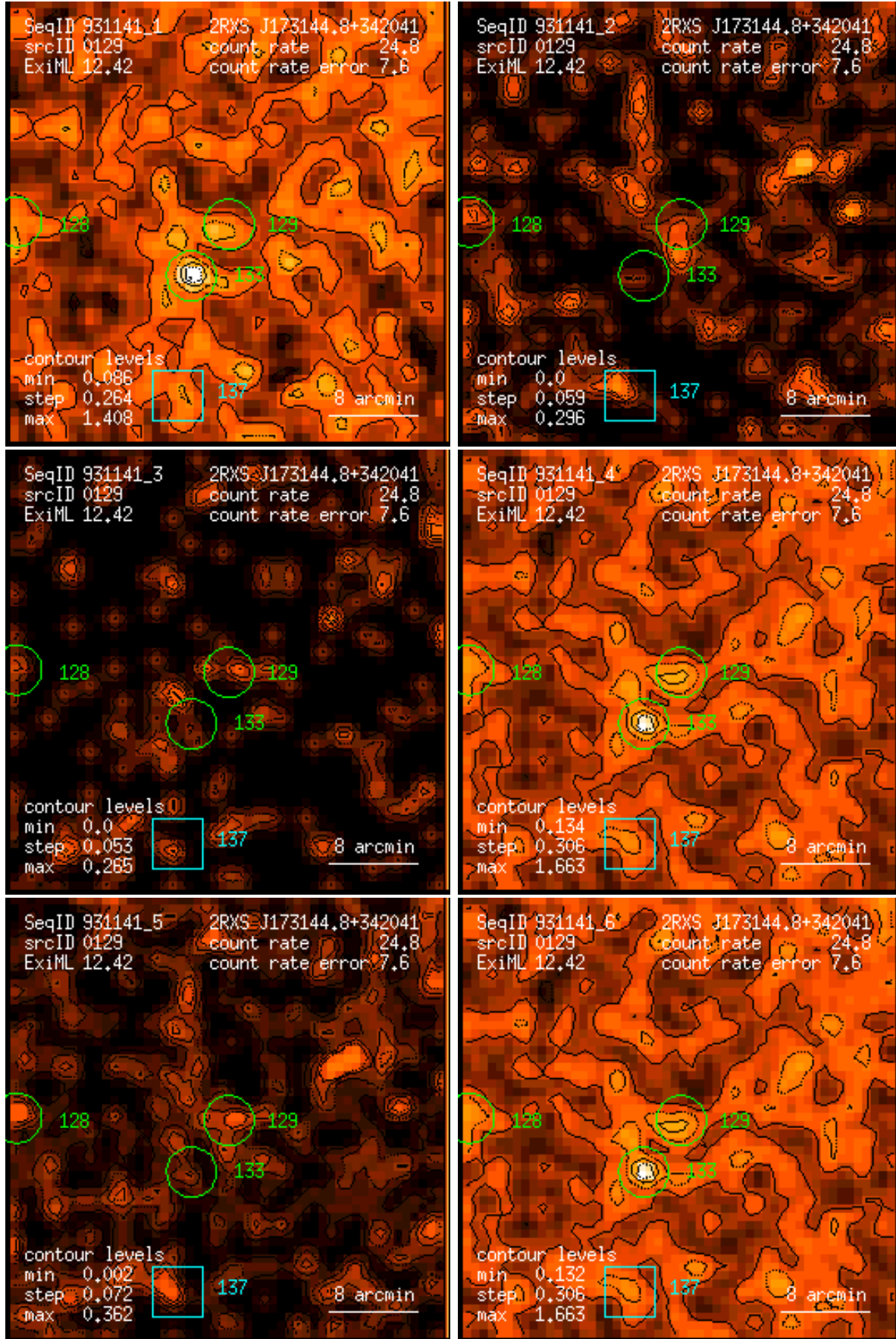
Figure 129: RASS 931141: detection 0129: band rate images, Gaussian filter: (1) PSPC channels 11 – 41, (2) 52 – 90, (3) 91 – 201, (4) 11 – 235, (5) 52 – 201, (6) 11 – 201. Broad band rates in counts/ks. Band rate contour levels in counts/ks/arcmin 2 .
