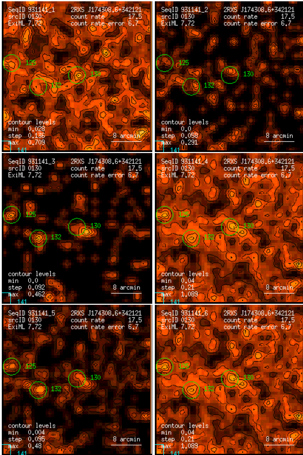
Figure 130: RASS 931141: detection 0130: band rate images, Gaussian filter: (1) PSPC channels 11 – 41, (2) 52 – 90, (3) 91 – 201, (4) 11 – 235, (5) 52 – 201, (6) 11 – 201. Broad band rates in counts/ks. Band rate contour levels in counts/ks/arcmin 2 .
