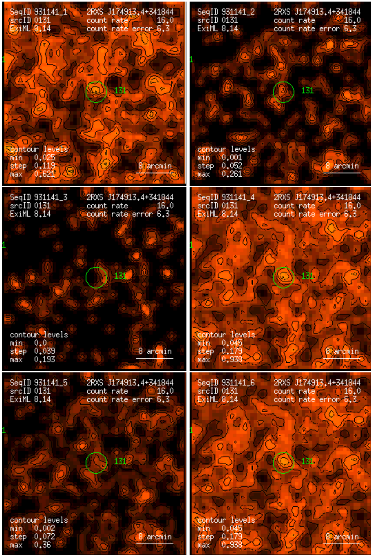
Figure 131: RASS 931141: detection 0131: band rate images, Gaussian filter: (1) PSPC channels 11 – 41, (2) 52 – 90, (3) 91 – 201, (4) 11 – 235, (5) 52 – 201, (6) 11 – 201. Broad band rates in counts/ks. Band rate contour levels in counts/ks/arcmin 2 .
