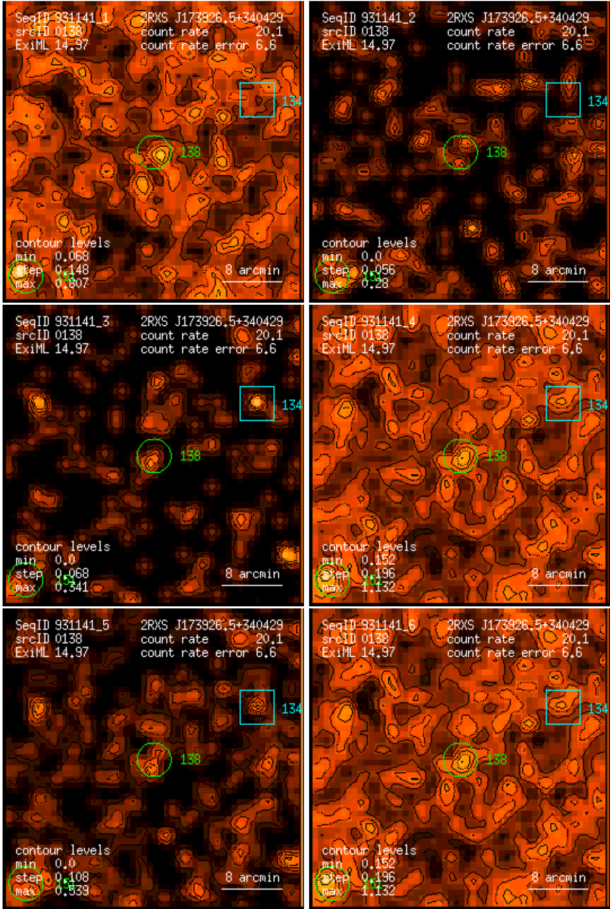
Figure 138: RASS 931141: detection 0138: band rate images, Gaussian filter: (1) PSPC channels 11 – 41, (2) 52 – 90, (3) 91 – 201, (4) 11 – 235, (5) 52 – 201, (6) 11 – 201. Broad band rates in counts/ks. Band rate contour levels in counts/ks/arcmin 2 .
