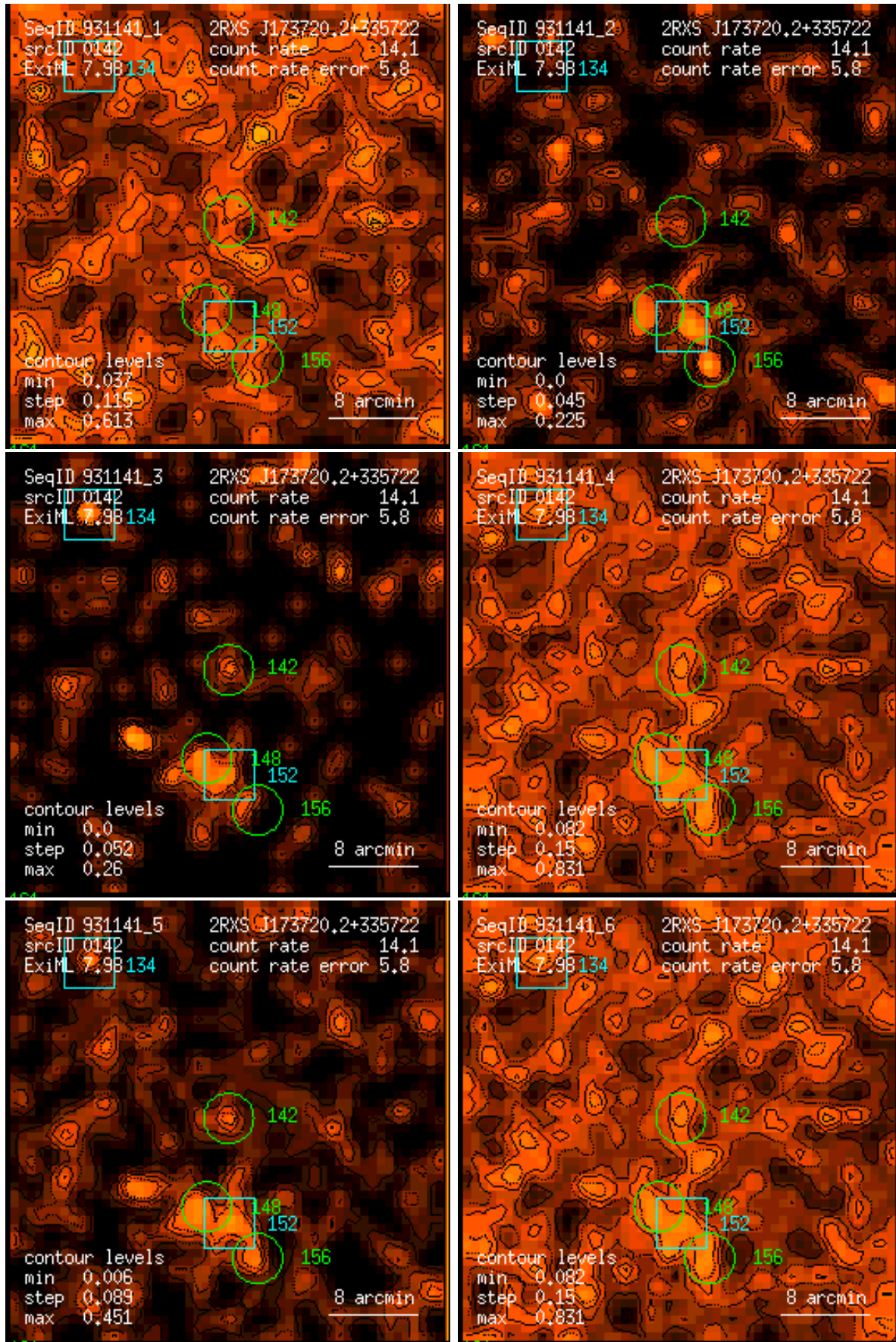
Figure 142: RASS 931141: detection 0142: band rate images, Gaussian filter: (1) PSPC channels 11 – 41, (2) 52 – 90, (3) 91 – 201, (4) 11 – 235, (5) 52 – 201, (6) 11 – 201. Broad band rates in counts/ks. Band rate contour levels in counts/ks/arcmin 2 .
