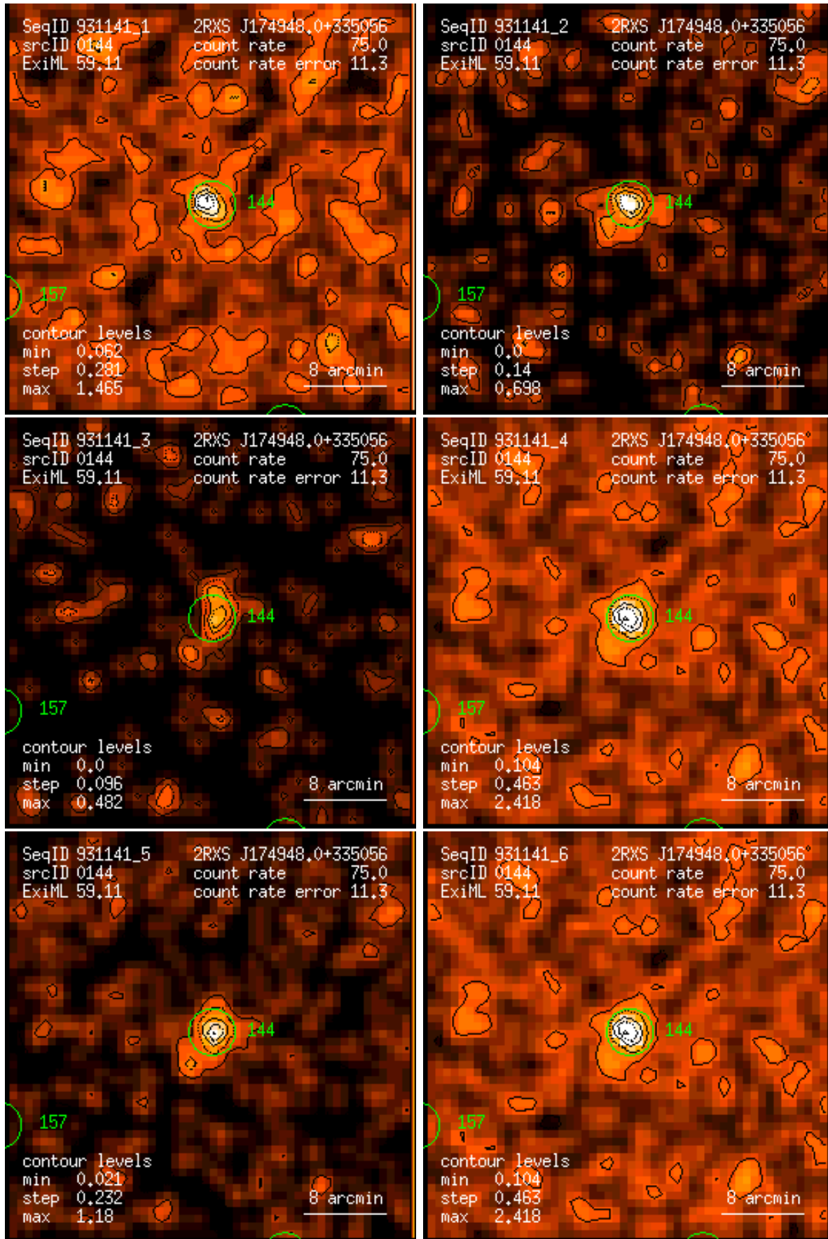
Figure 144: RASS 931141: detection 0144: band rate images, Gaussian filter: (1) PSPC channels 11 – 41, (2) 52 – 90, (3) 91 – 201, (4) 11 – 235, (5) 52 – 201, (6) 11 – 201. Broad band rates in counts/ks. Band rate contour levels in counts/ks/arcmin 2 .
