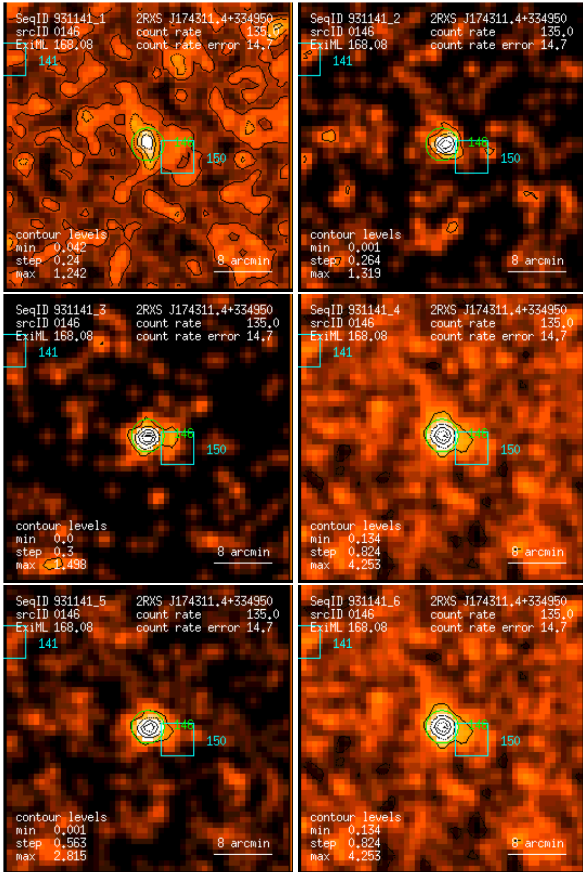
Figure 146: RASS 931141: detection 0146: band rate images, Gaussian filter: (1) PSPC channels 11 – 41, (2) 52 – 90, (3) 91 – 201, (4) 11 – 235, (5) 52 – 201, (6) 11 – 201. Broad band rates in counts/ks. Band rate contour levels in counts/ks/arcmin 2 .
