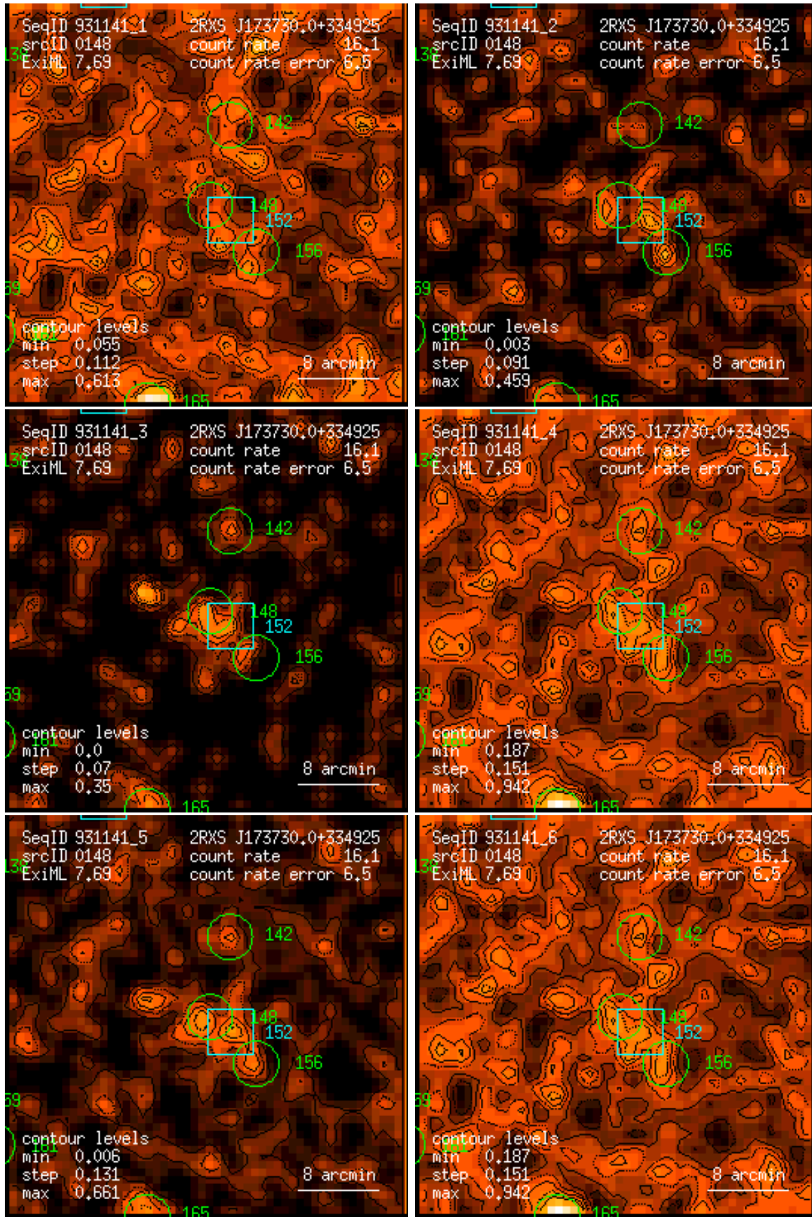
Figure 148: RASS 931141: detection 0148: band rate images, Gaussian filter: (1) PSPC channels 11 – 41, (2) 52 – 90, (3) 91 – 201, (4) 11 – 235, (5) 52 – 201, (6) 11 – 201. Broad band rates in counts/ks. Band rate contour levels in counts/ks/arcmin 2 .
