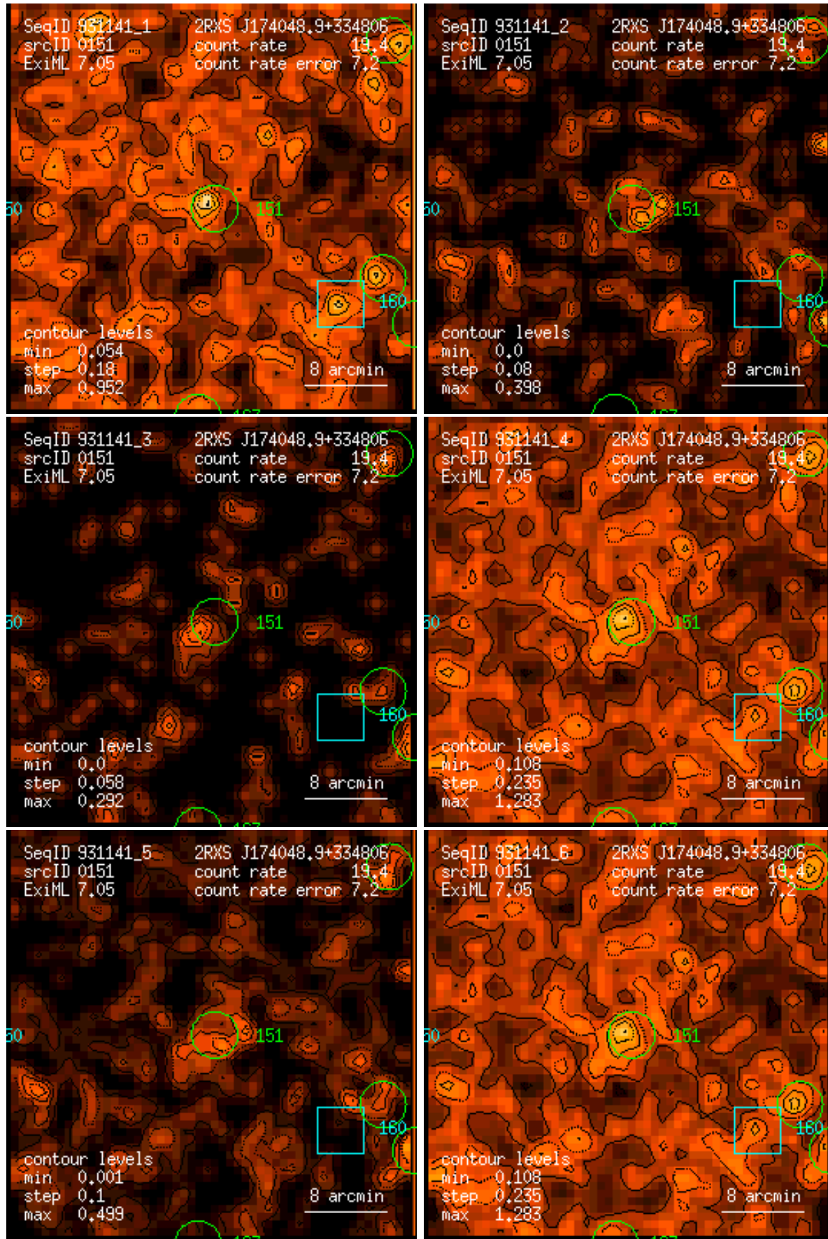
Figure 151: RASS 931141: detection 0151: band rate images, Gaussian filter: (1) PSPC channels 11 – 41, (2) 52 – 90, (3) 91 – 201, (4) 11 – 235, (5) 52 – 201, (6) 11 – 201. Broad band rates in counts/ks. Band rate contour levels in counts/ks/arcmin 2 .
