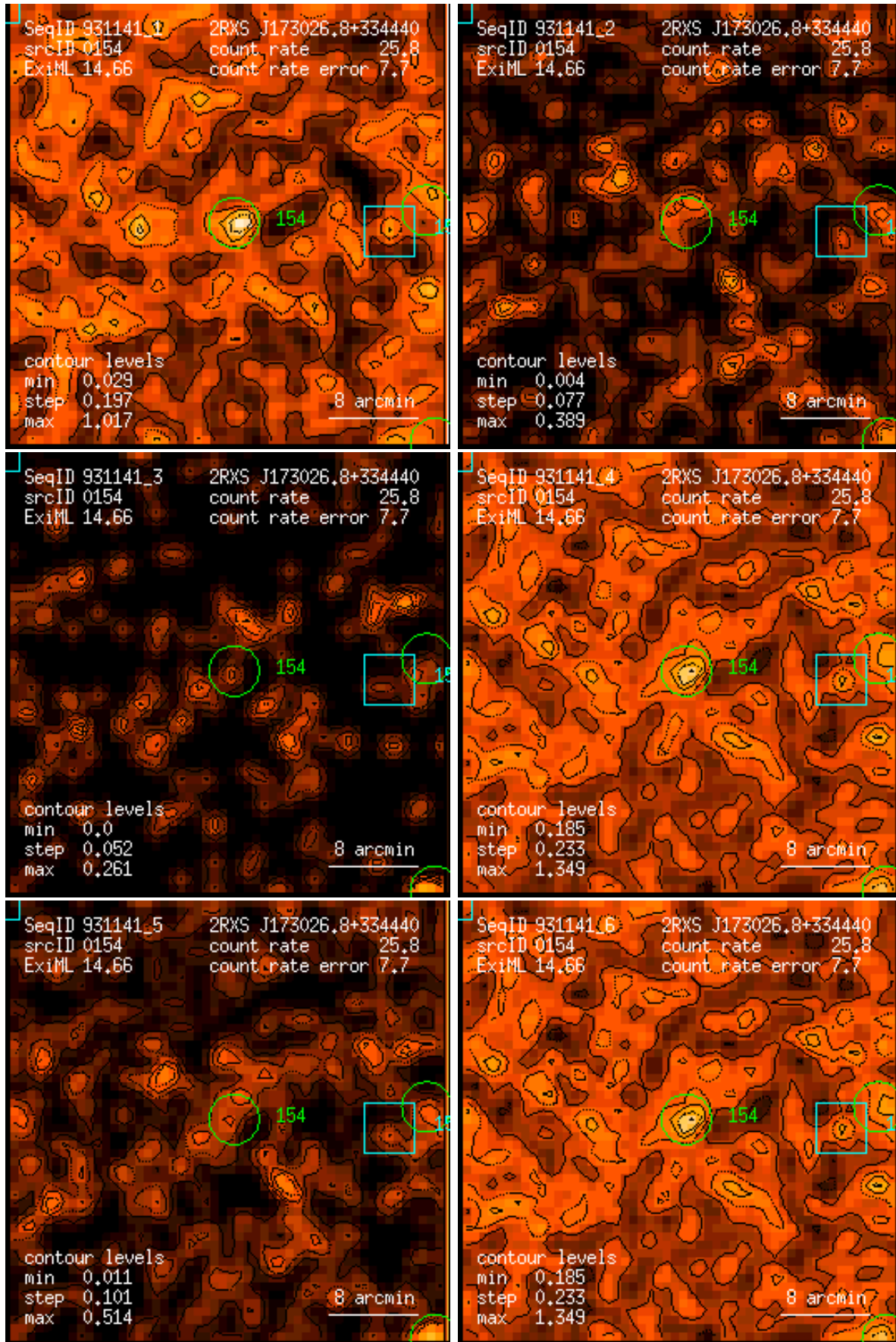
Figure 154: RASS 931141: detection 0154: band rate images, Gaussian filter: (1) PSPC channels 11 – 41, (2) 52 – 90, (3) 91 – 201, (4) 11 – 235, (5) 52 – 201, (6) 11 – 201. Broad band rates in counts/ks. Band rate contour levels in counts/ks/arcmin 2 .
