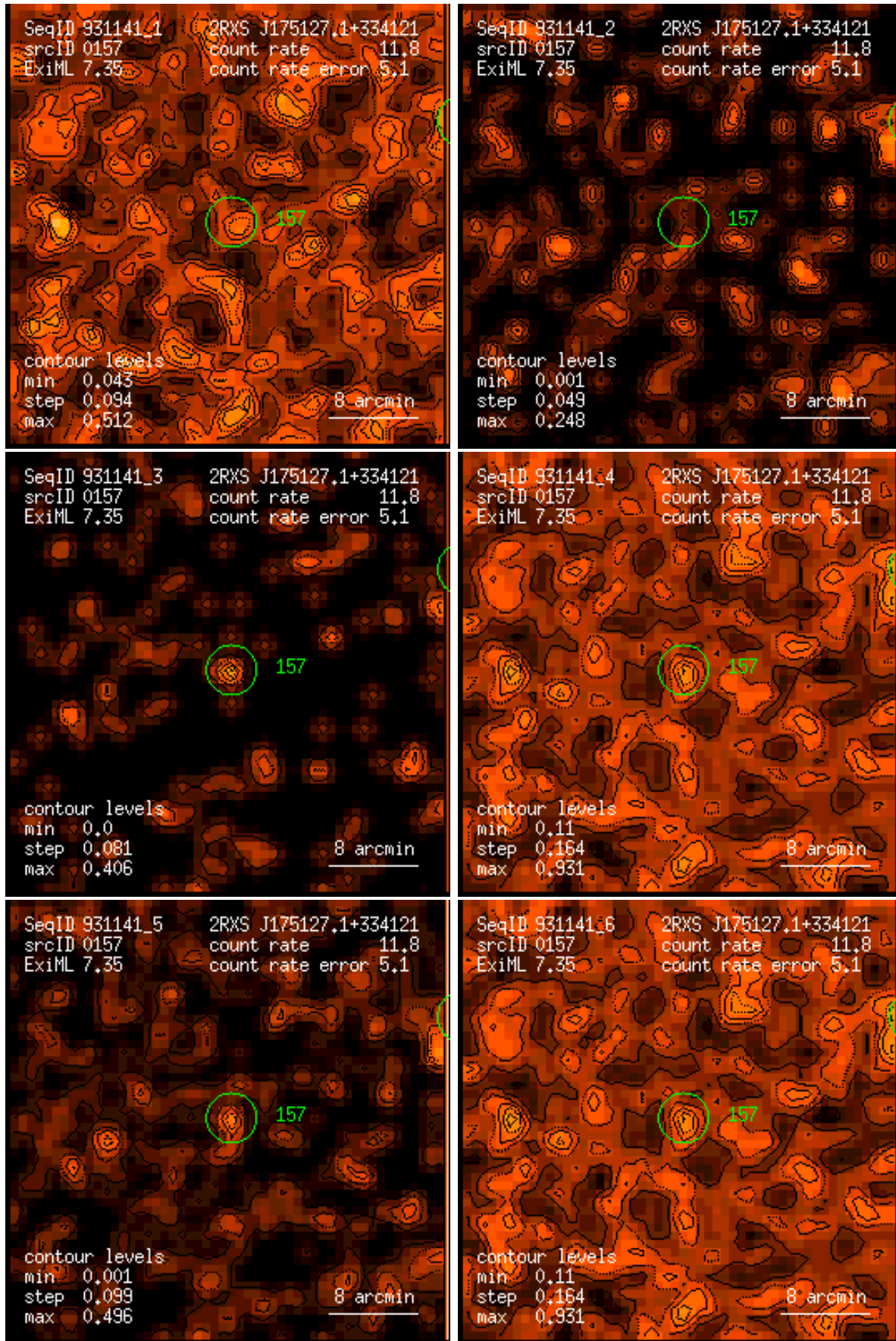
Figure 157: RASS 931141: detection 0157: band rate images, Gaussian filter: (1) PSPC channels 11 – 41, (2) 52 – 90, (3) 91 – 201, (4) 11 – 235, (5) 52 – 201, (6) 11 – 201. Broad band rates in counts/ks. Band rate contour levels in counts/ks/arcmin 2 .
